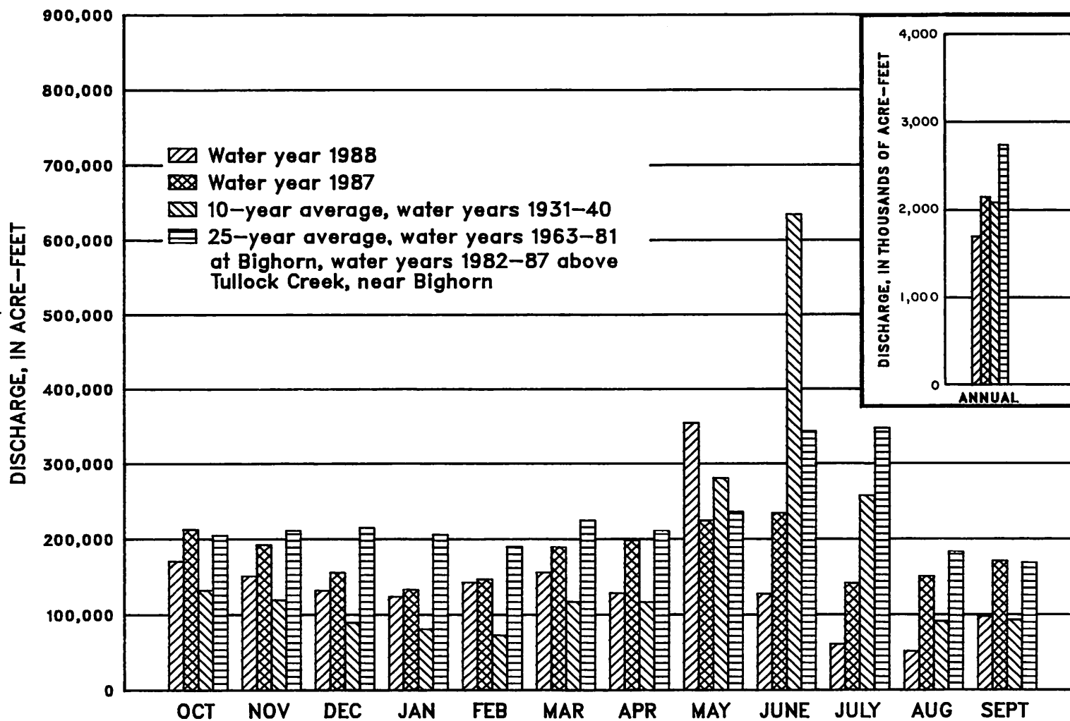
Figure 2.--Comparison of discharge for water year 1988 with discharge for water year 1987 of Bighorn River above Tullock Creek, near Bighorn and with average discharge for water years 1931-40 and 1963-81 at Bighorn and 1982-87 above Tullock Creek, near Bighorn.
