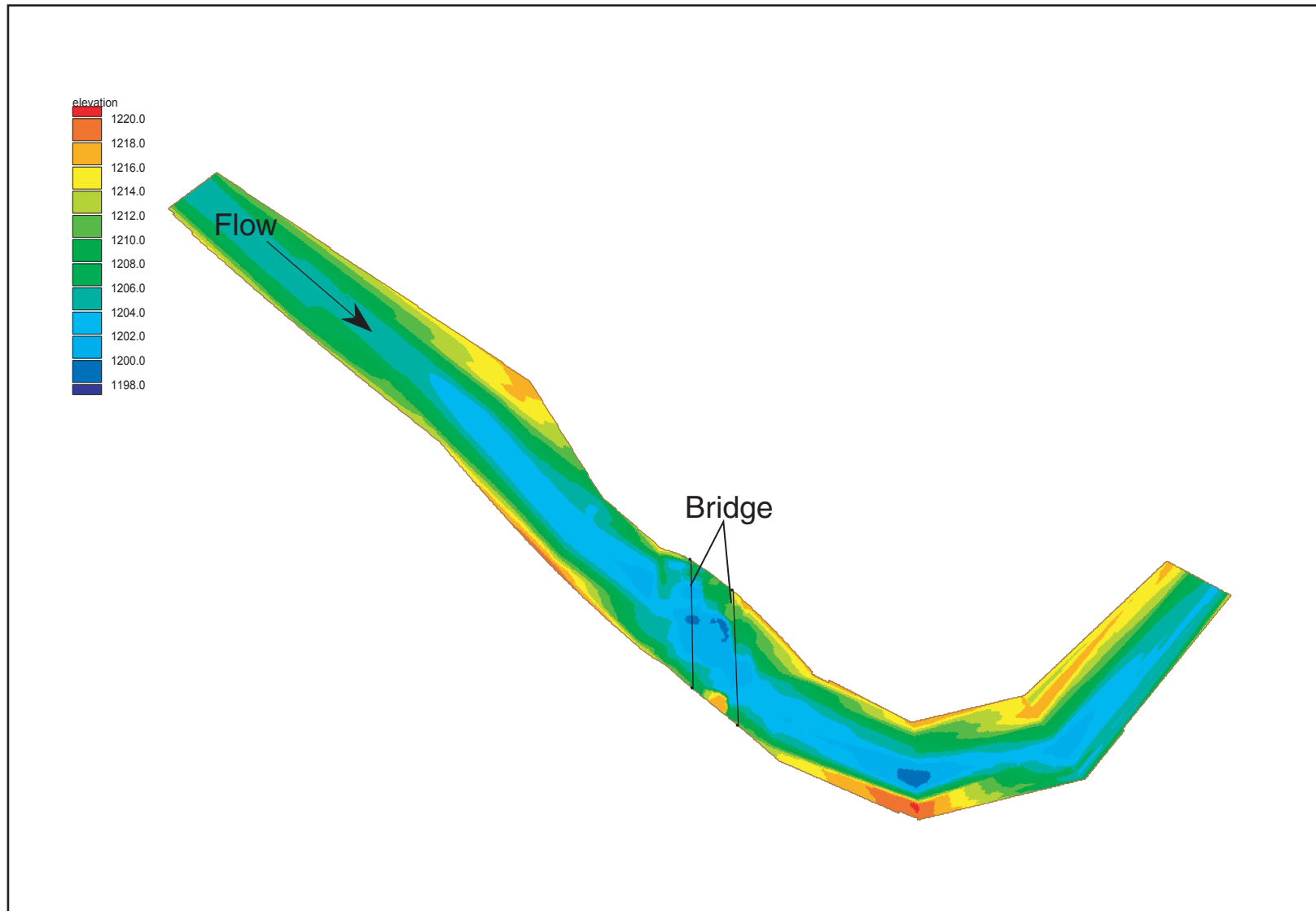
Figure 3. - James River bathymetry throughout SR 37 bridge reach, collected during April 2001 flood
