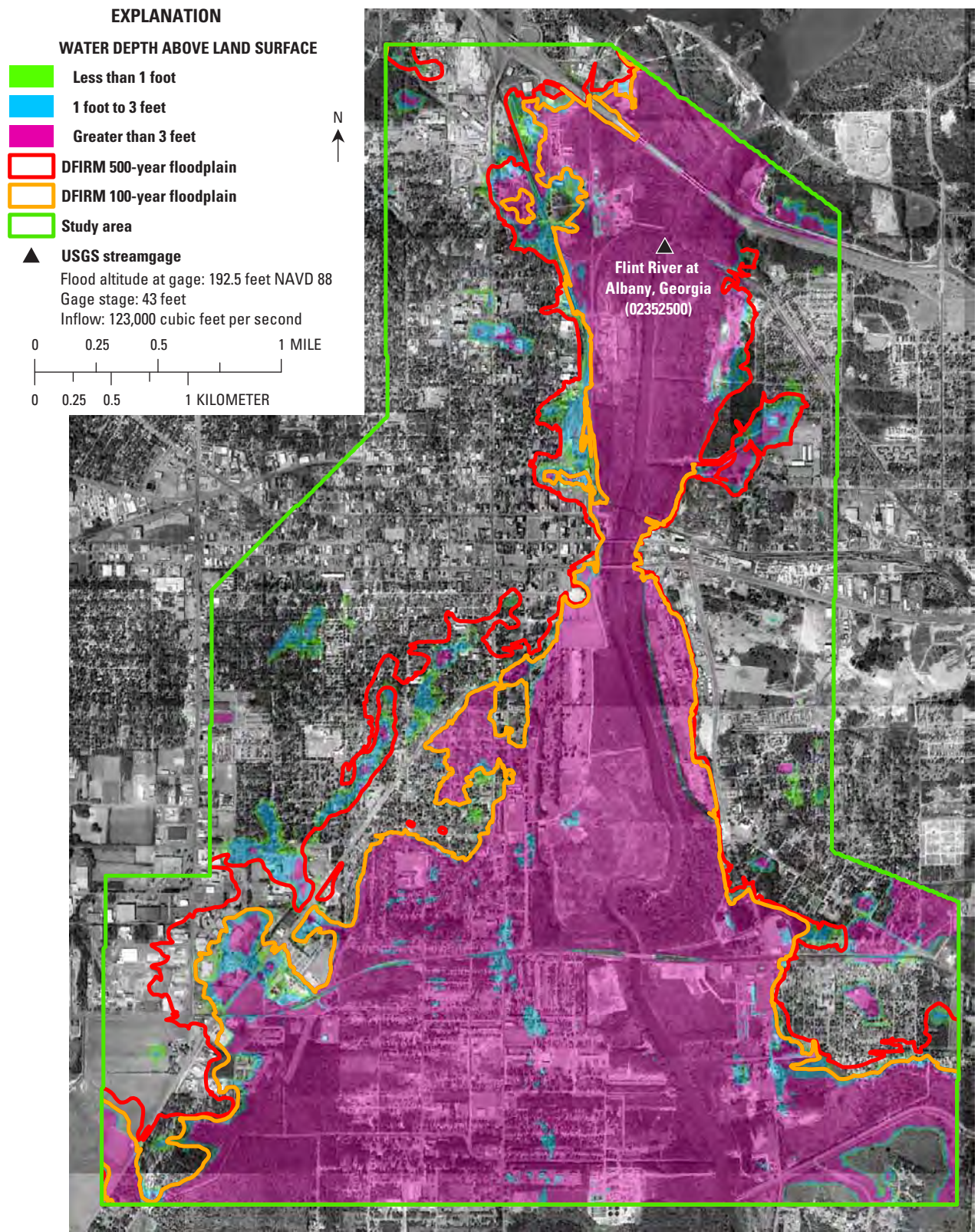
Figure A28. Simulated flood-inundation hazard scale for a water-surface altitude of 192.5 feet at the Albany streamgage compared with Federal Emergency Management Agency’s Digital Flood Insurance Rate Maps (DFIRM) for the Flint River in Albany, Georgia, 1998.
