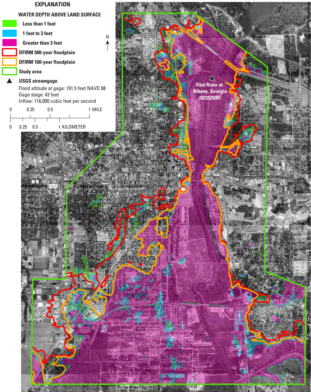
Figure A27. Simulated flood-inundation hazard scale for a water-surface altitude of 191.5 feet at the Albany streamgage compared with Federal Emergency Management Agency’s Digital Flood Insurance Rate Maps (DFIRM) for the Flint River in Albany, Georgia, 1998.
