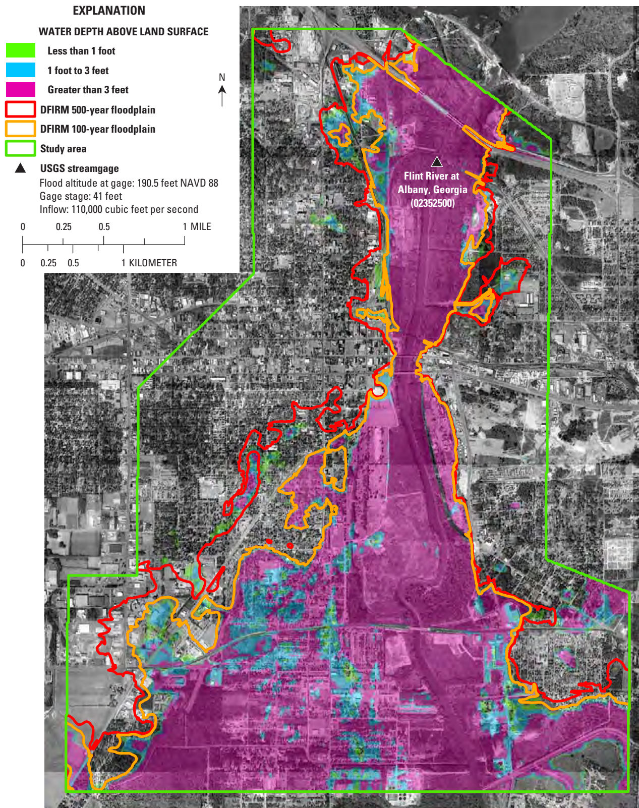
Figure A26. Simulated flood-inundation hazard scale for a water-surface altitude of 190.5 feet at the Albany streamgage compared with Federal Emergency Management Agency’s Digital Flood Insurance Rate Maps (DFIRM) for the Flint River in Albany, Georgia, 1998.
