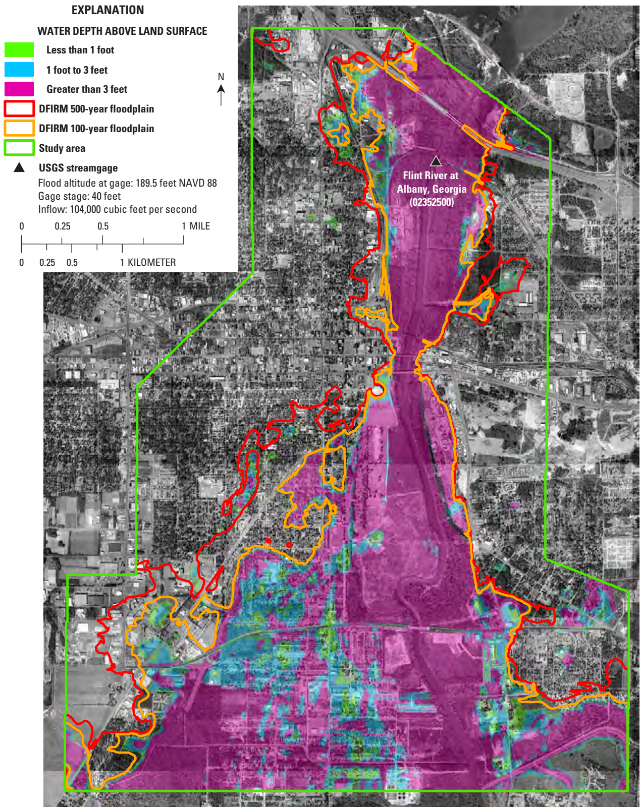
Figure A25. Simulated flood-inundation hazard scale for a water-surface altitude of 189.5 feet at the Albany streamgage compared with Federal Emergency Management Agency’s Digital Flood Insurance Rate Maps (DFIRM) for the Flint River in Albany, Georgia, 1998.
