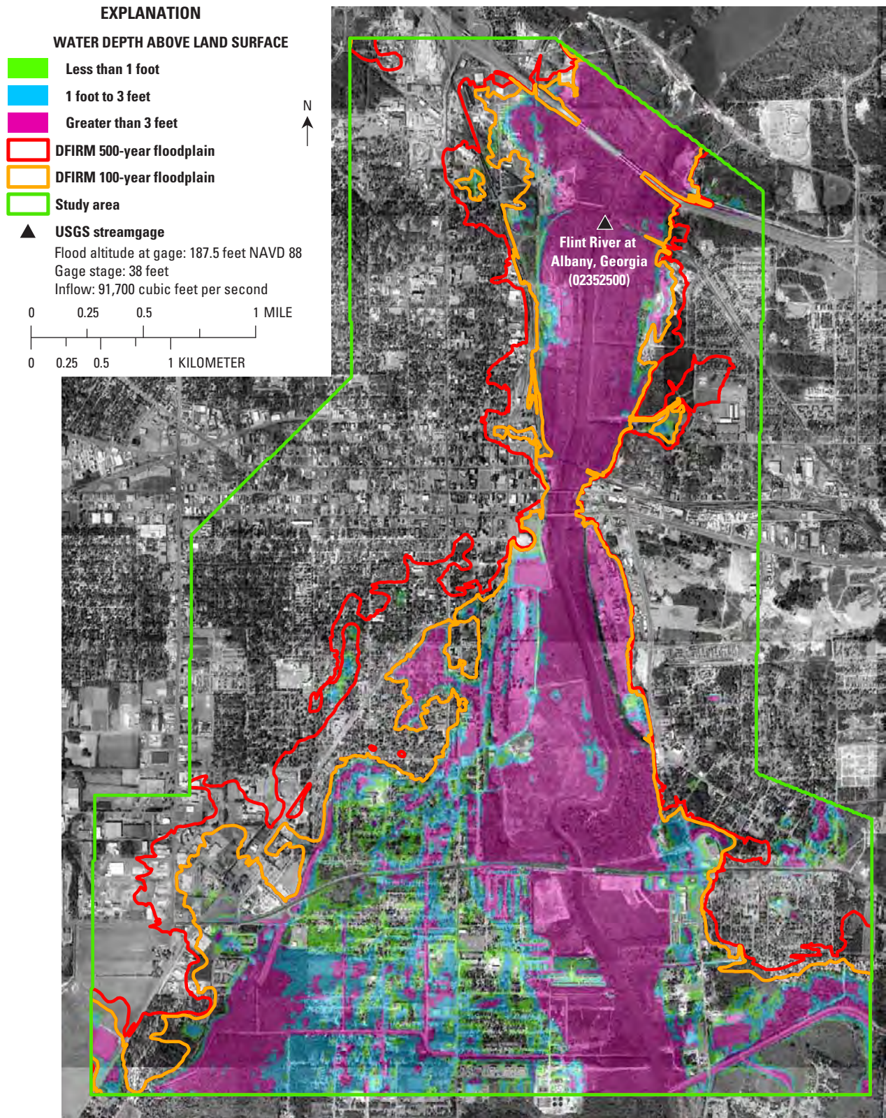
Figure A23. Simulated flood-inundation hazard scale for a water-surface altitude of 187.5 feet at the Albany streamgage compared with Federal Emergency Management Agency’s Digital Flood Insurance Rate Maps (DFIRM) for the Flint River in Albany, Georgia, 1998.
