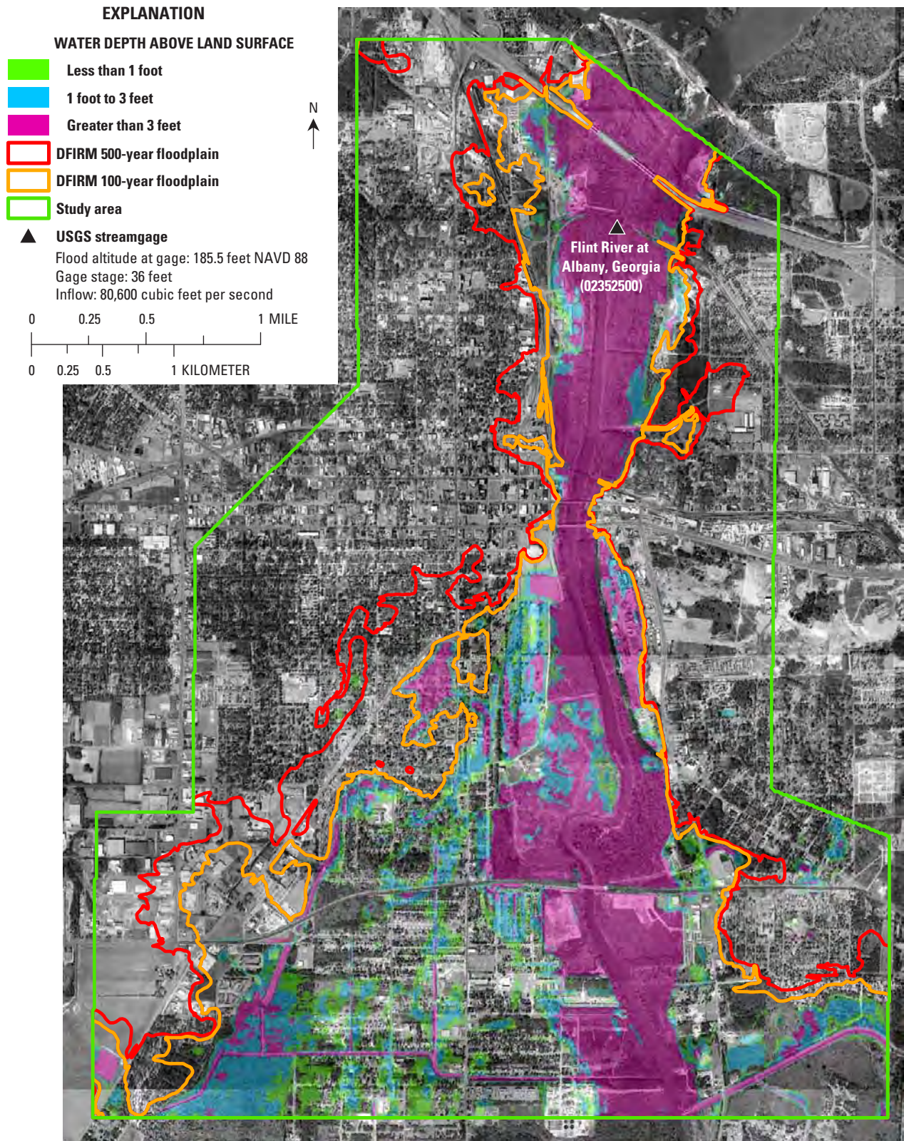
Figure A21. Simulated flood-inundation hazard scale for a water-surface altitude of 185.5 feet at the Albany streamgage compared with Federal Emergency Management Agency’s Digital Flood Insurance Rate Maps (DFIRM) for the Flint River in Albany, Georgia, 1998.
