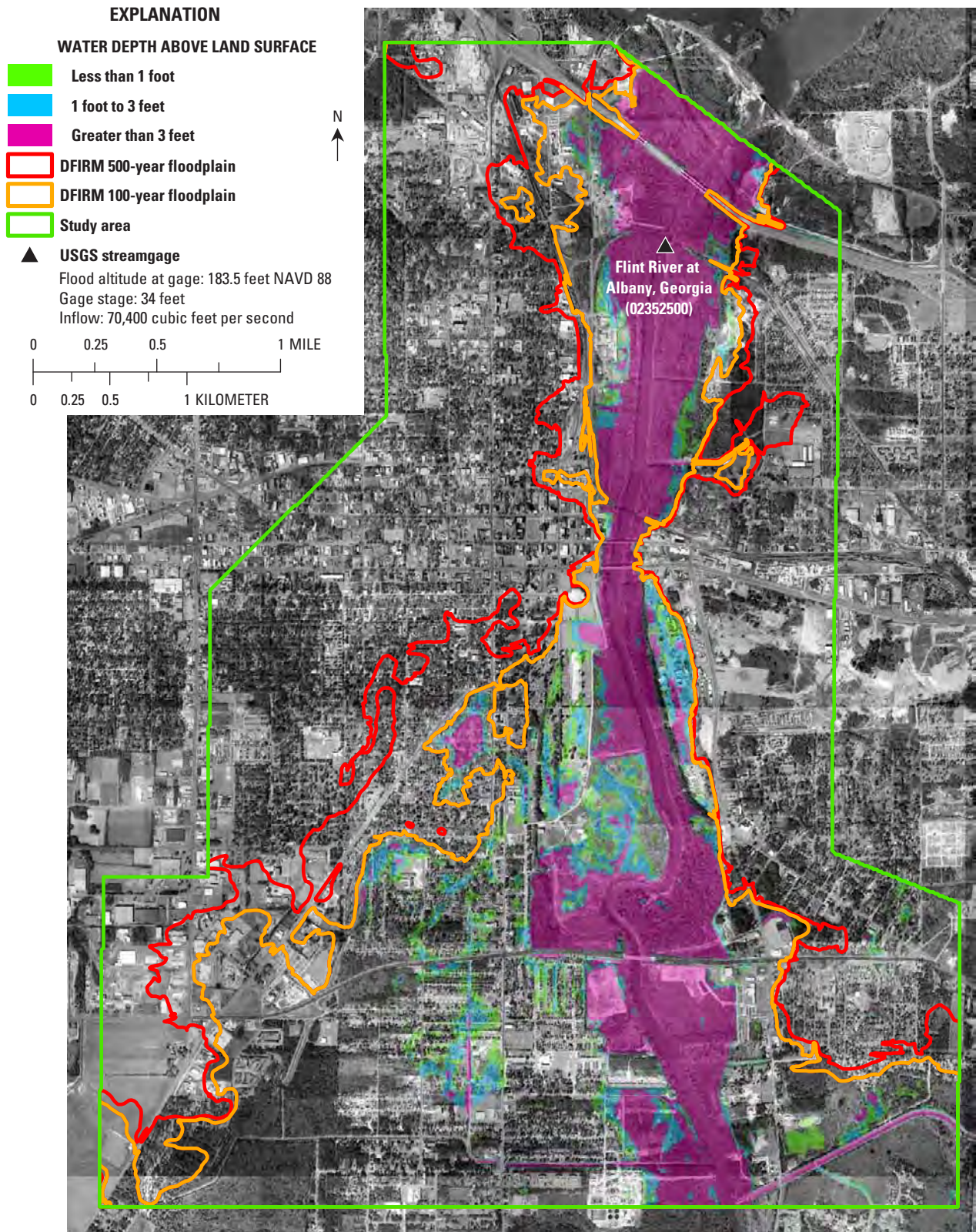
Figure A19. Simulated flood-inundation hazard scale for a water-surface altitude of 183.5 feet at the Albany streamgage compared with Federal Emergency Management Agency’s Digital Flood Insurance Rate Maps (DFIRM) for the Flint River in Albany, Georgia, 1998.
