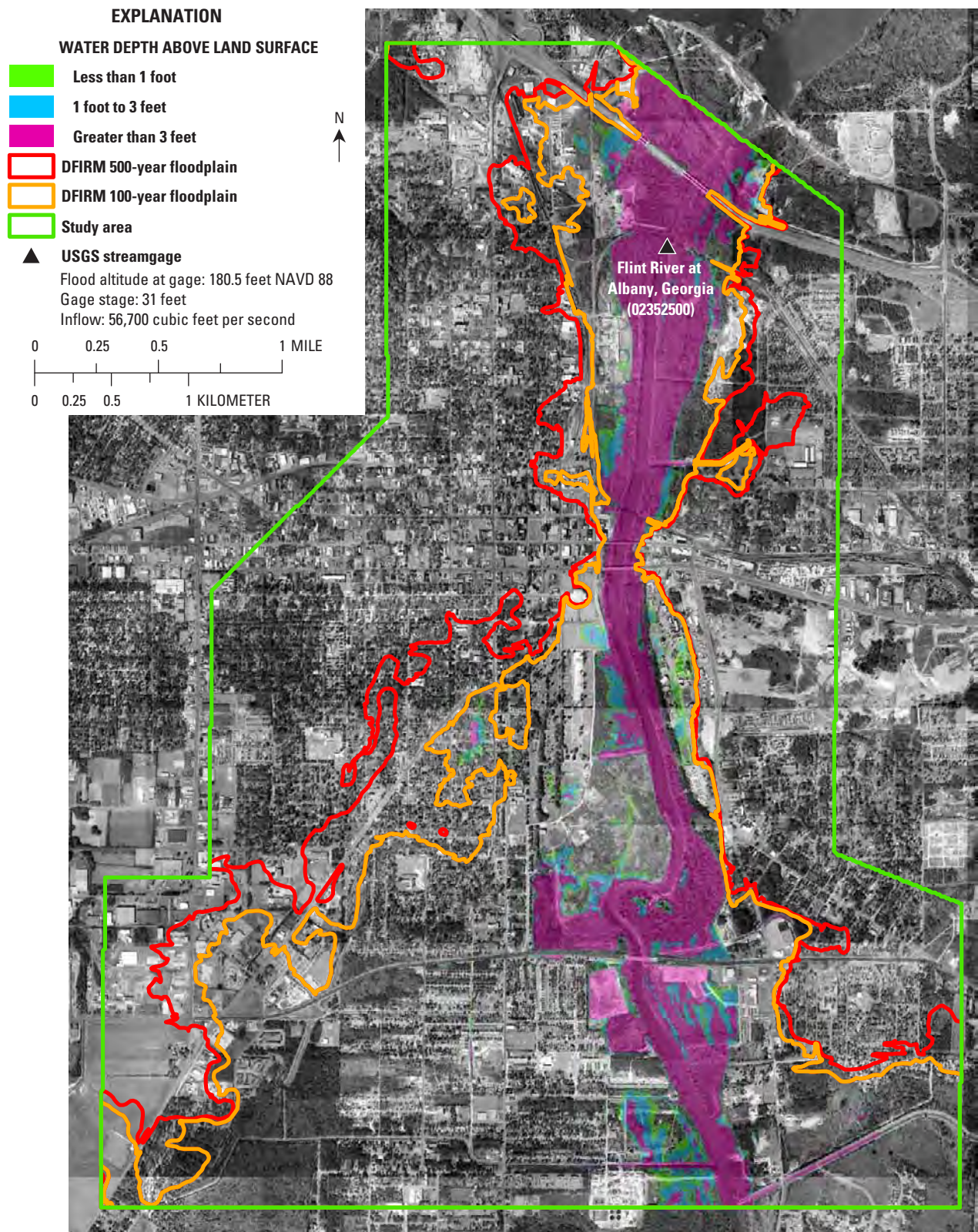
Figure A16. Simulated flood-inundation hazard scale for a water-surface altitude of 180.5 feet at the Albany streamgage compared with Federal Emergency Management Agency’s Digital Flood Insurance Rate Maps (DFIRM) for the Flint River in Albany, Georgia, 1998.
