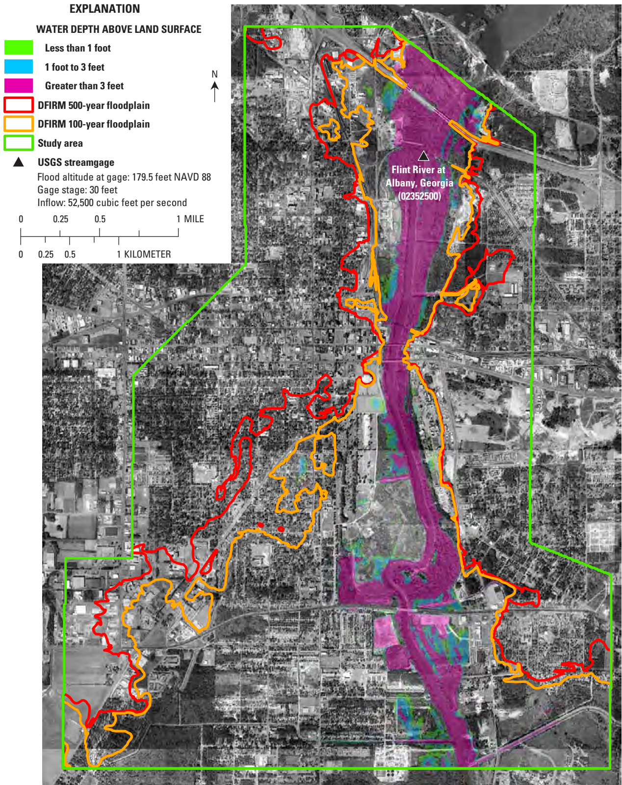
Figure A15. Simulated flood-inundation hazard scale for a water-surface altitude of 179.5 feet at the Albany streamgage compared with Federal Emergency Management Agency’s Digital Flood Insurance Rate Maps (DFIRM) for the Flint River in Albany, Georgia, 1998.
