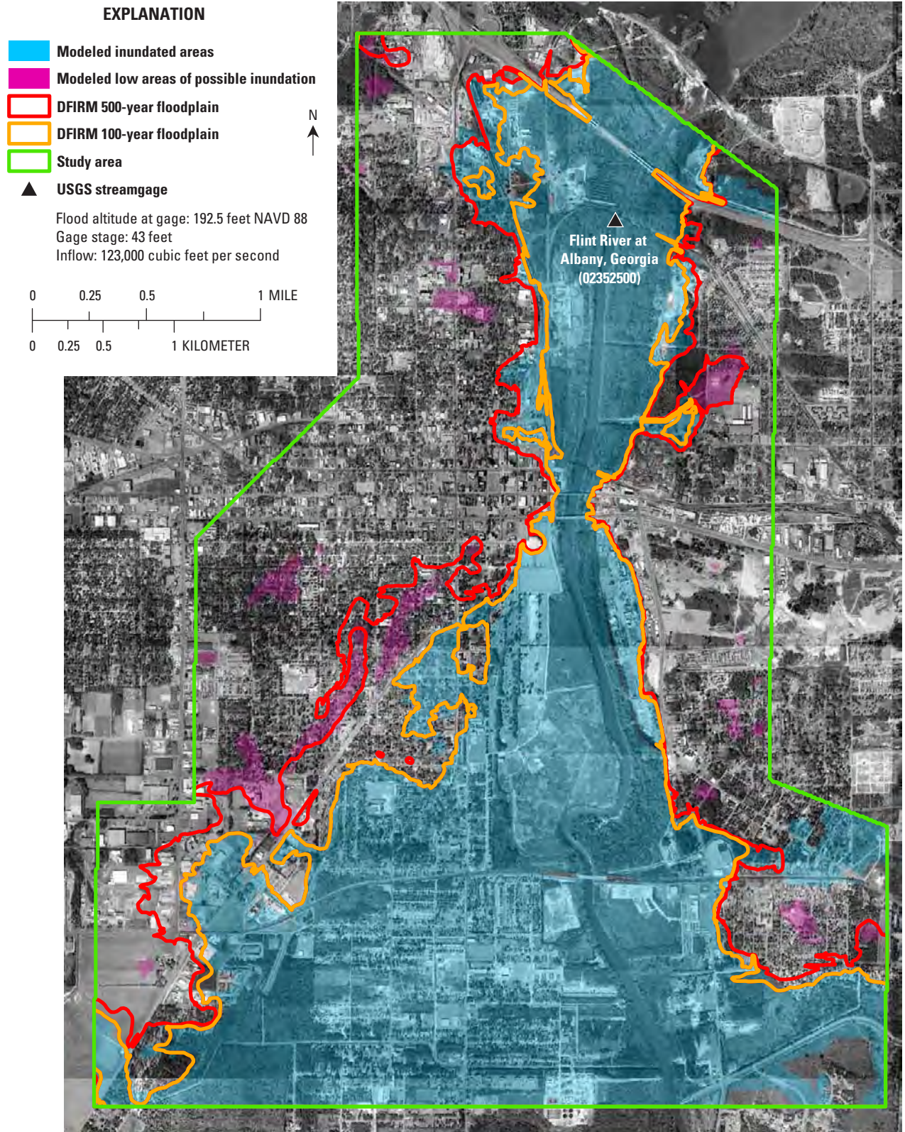
Figure A14. Simulated flood inundation for a water-surface altitude of 192.5 feet at the Albany streamgauge compared with Federal Emergency Management Agency’s Digital Flood Insurance Rate Maps (DFIRM) for the Flint River in Albany, Georgia, 1998.
