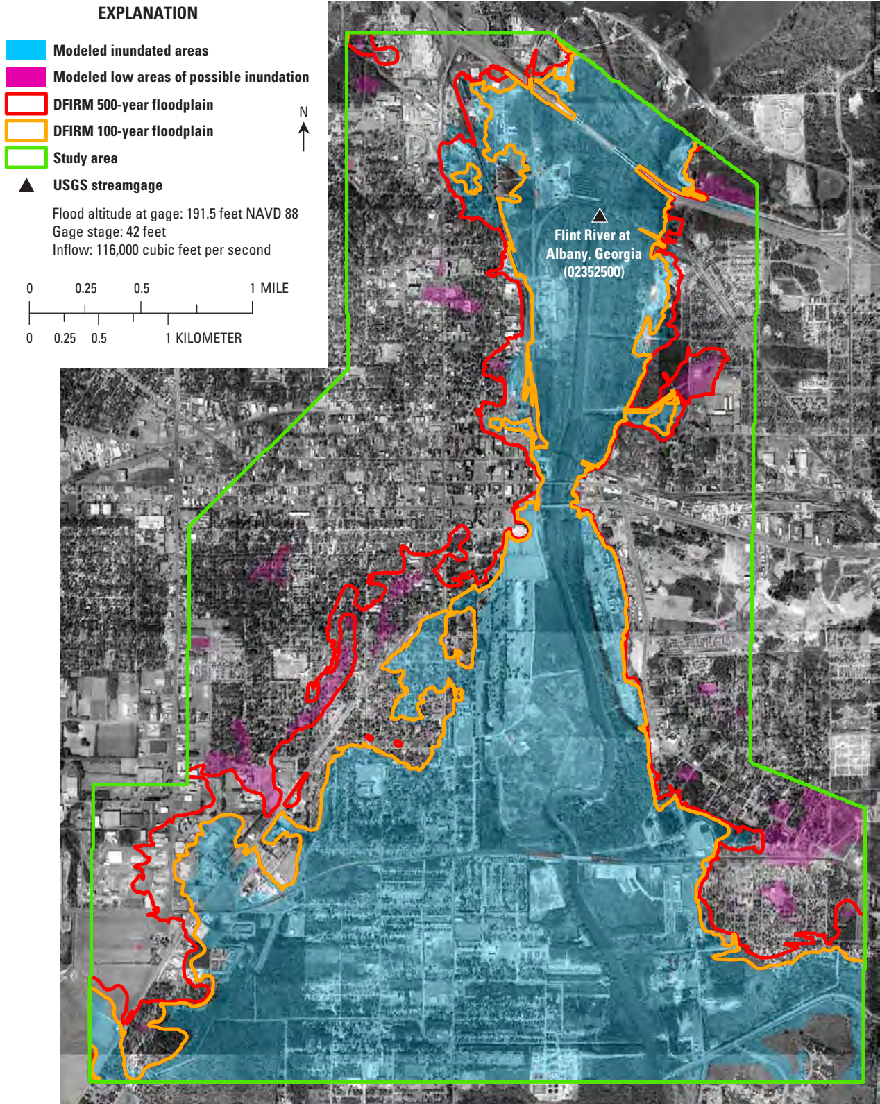
Figure A13. Simulated flood inundation for a water-surface altitude of 191.5 feet at the Albany streamgage compared with Federal Emergency Management Agency’s Digital Flood Insurance Rate Maps (DFIRM) for the Flint River in Albany, Georgia, 1998.
