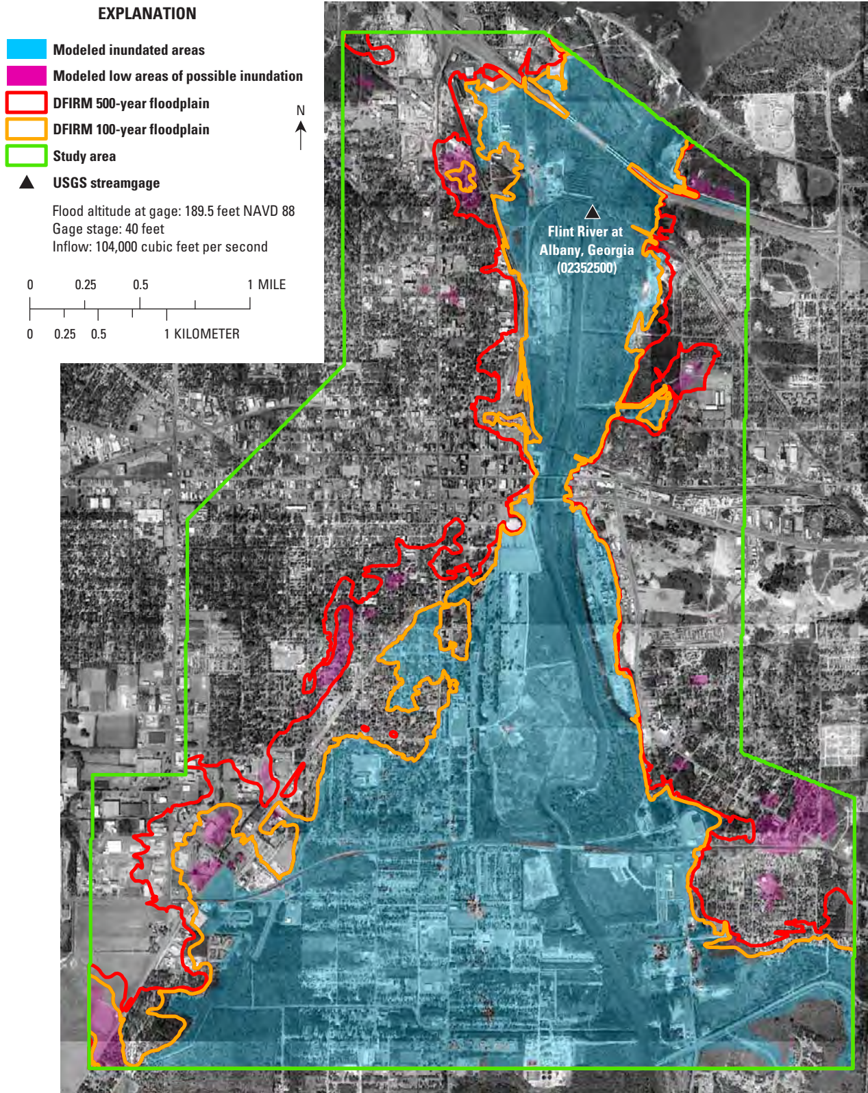
Figure A11. Simulated flood inundation for a water-surface altitude of 189.5 feet at the Albany streamgage compared with Federal Emergency Management Agency's Digital Flood Insurance Rate Maps (DFIRM) for the Flint River in Albany, Georgia, 1998.
