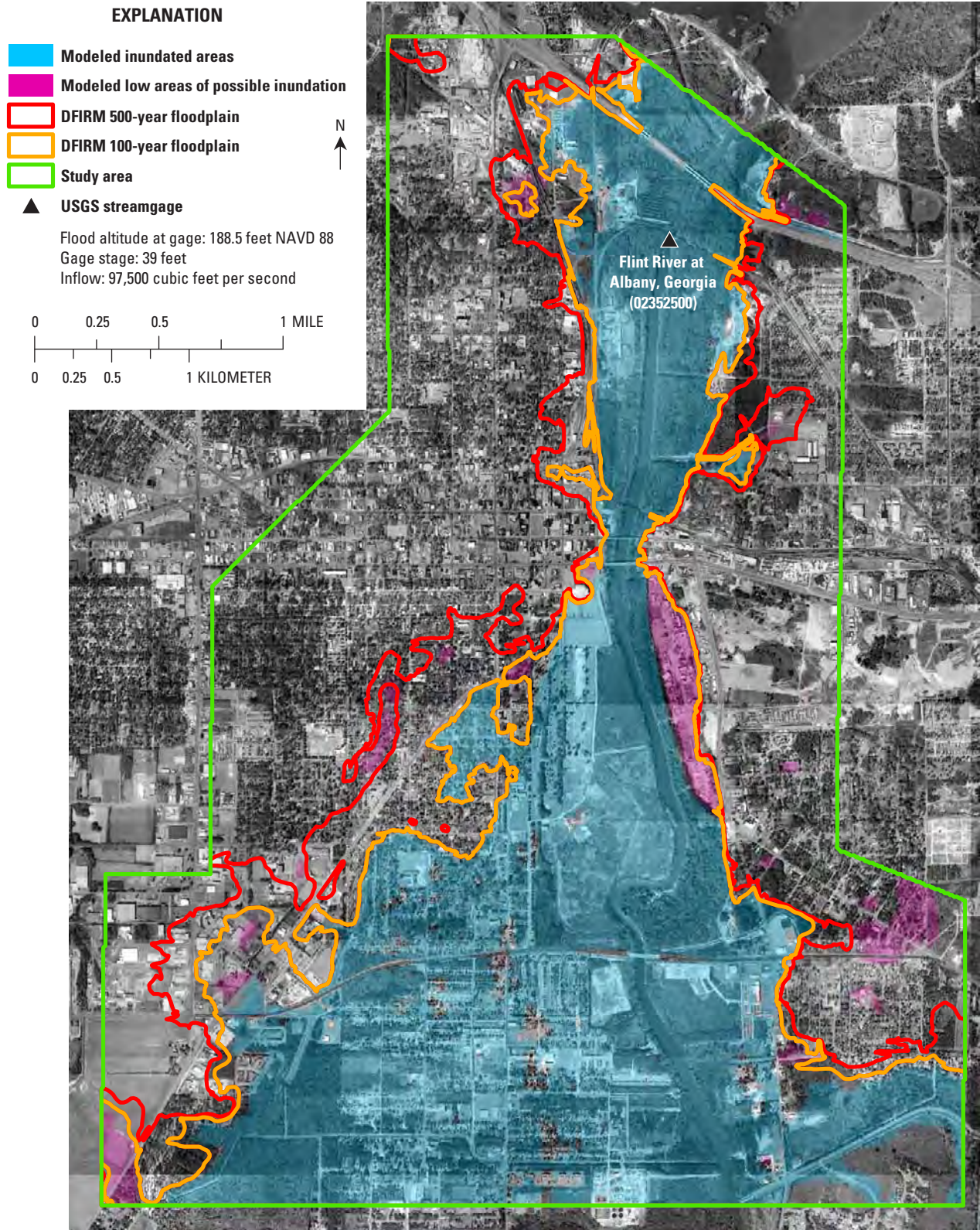
Figure A10. Simulated flood inundation for a water-surface altitude of 188.5 feet at the Albany streamgage compared with Federal Emergency Management Agency’s Digital Flood Insurance Rate Maps (DFIRM) for the Flint River in Albany, Georgia, 1998.
