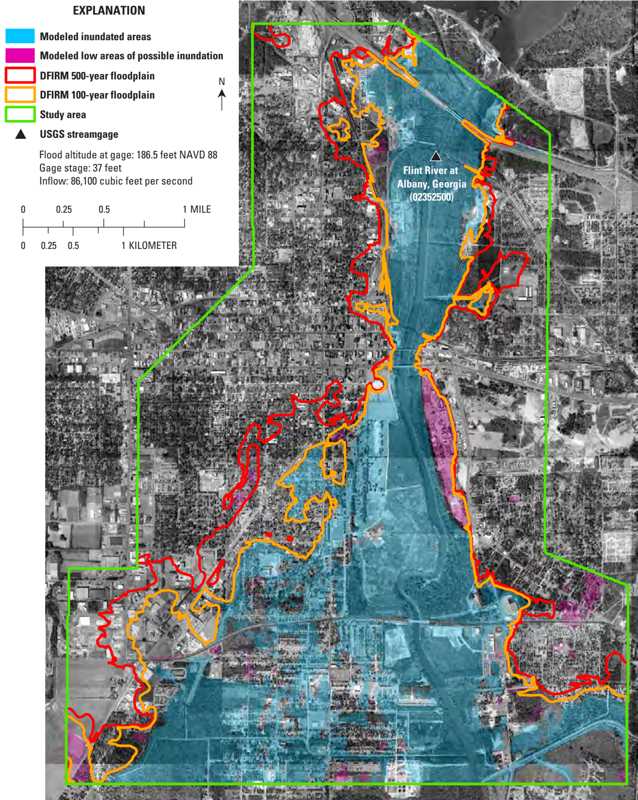
Figure A8. Simulated flood inundation for a water-surface altitude of 186.5 feet at the Albany streamgage compared with Federal Emergency Management Agency’s Digital Flood Insurance Rate Maps (DFIRM) for the Flint River in Albany, Georgia, 1998.
