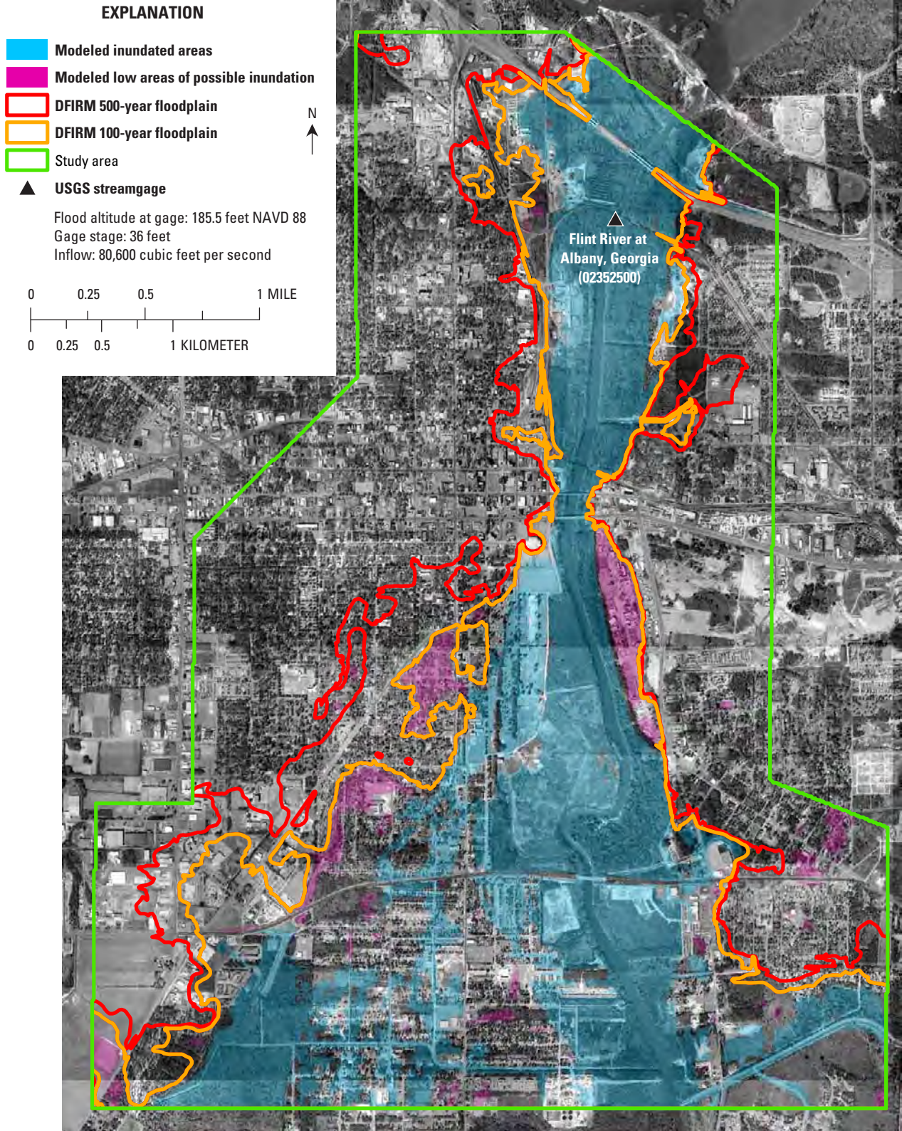
Figure A7. Simulated flood inundation for a water-surface altitude of 185.5 feet at the Albany streamgage compared with Federal Emergency Management Agency’s Digital Flood Insurance Rate Maps (DFIRM) for the Flint River in Albany, Georgia, 1998.
