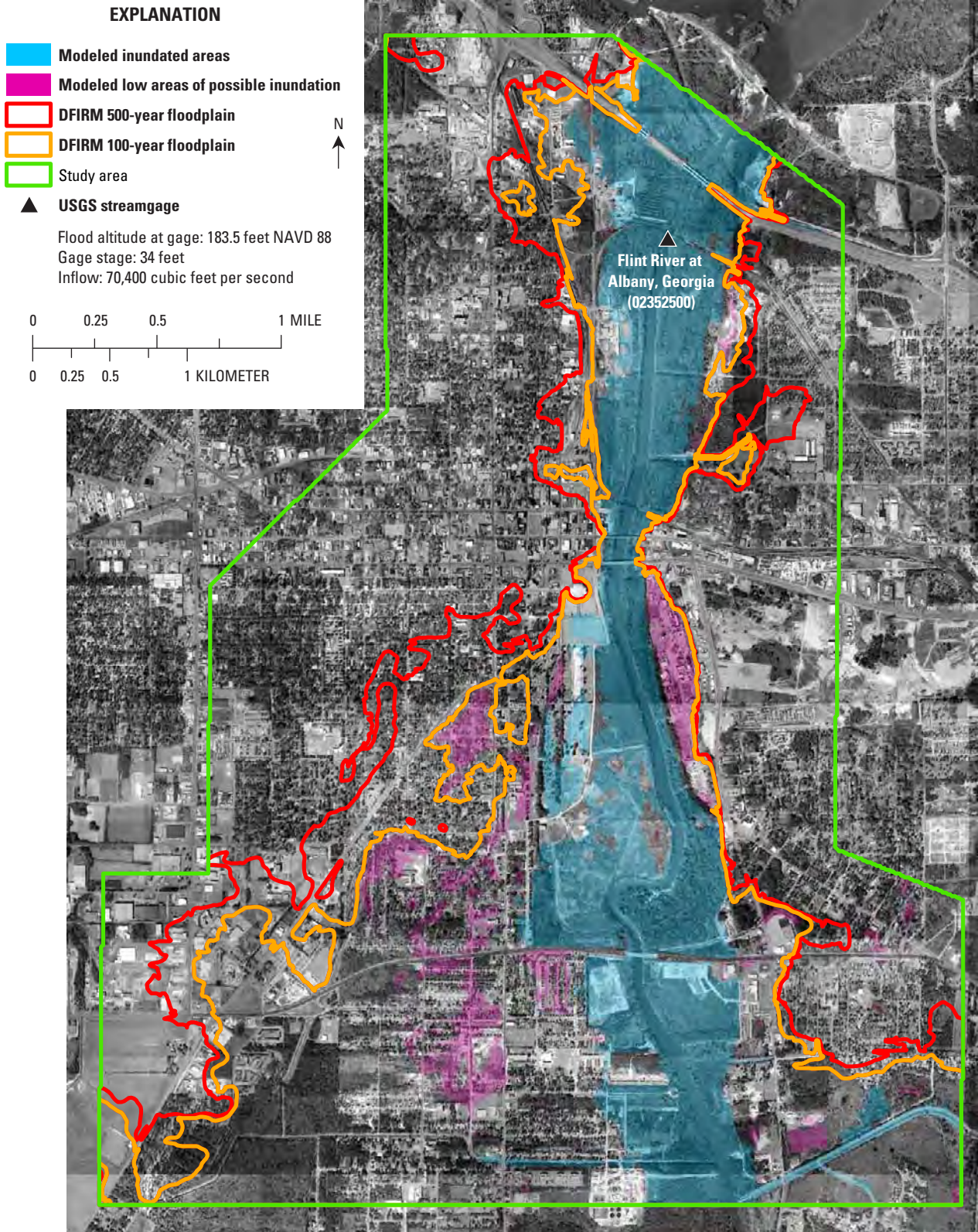
Figure A5. Simulated flood inundation for a water-surface altitude of 183.5 feet at the Albany streamgage compared with Federal Emergency Management Agency’s Digital Flood Insurance Rate Maps (DFIRM) for the Flint River in Albany, Georgia, 1998.
