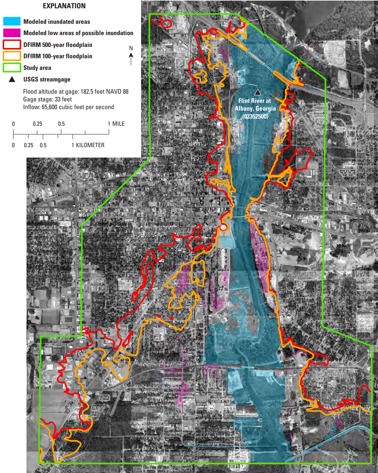
Figure A4. Simulated flood inundation for a water-surface altitude of 182.5 feet at the Albany streamgage compared with Federal Emergency Management Agency’s Digital Flood Insurance Rate Maps (DFIRM) for the Flint River in Albany, Georgia, 1998.
