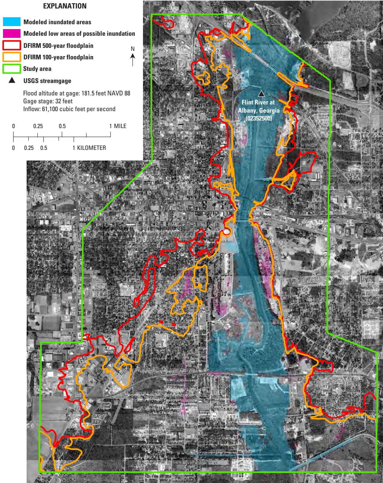
Figure A3. Simulated flood inundation for a water-surface altitude of 181.5 feet at the Albany streamgage compared with Federal Emergency Management Agency’s Digital Flood Insurance Rate Maps (DFIRM) for the Flint River in Albany, Georgia, 1998.
