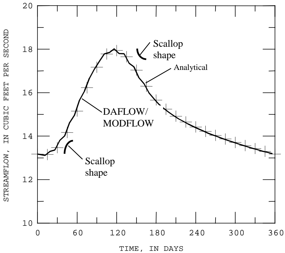
Figure 13. Simulated streamflow at node 14 and the analytical solution.
