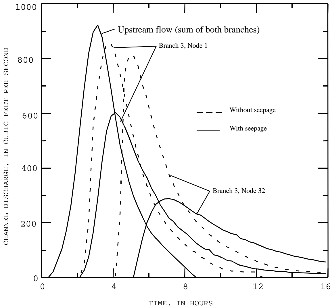
Figure 24. Flow distribution at selected points of the channel in example 3, illustrating the bank-storage effect on the flow hydrograph.
