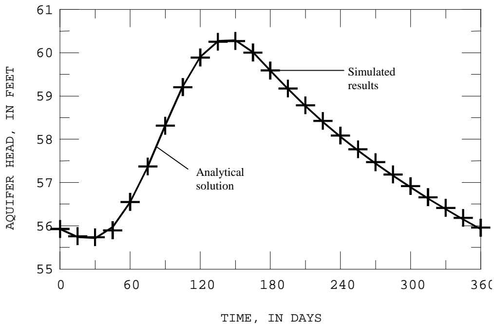
Figure 14. The simulated and analytical variation of water level in a well located in row 7, column 10 of figure 8.
