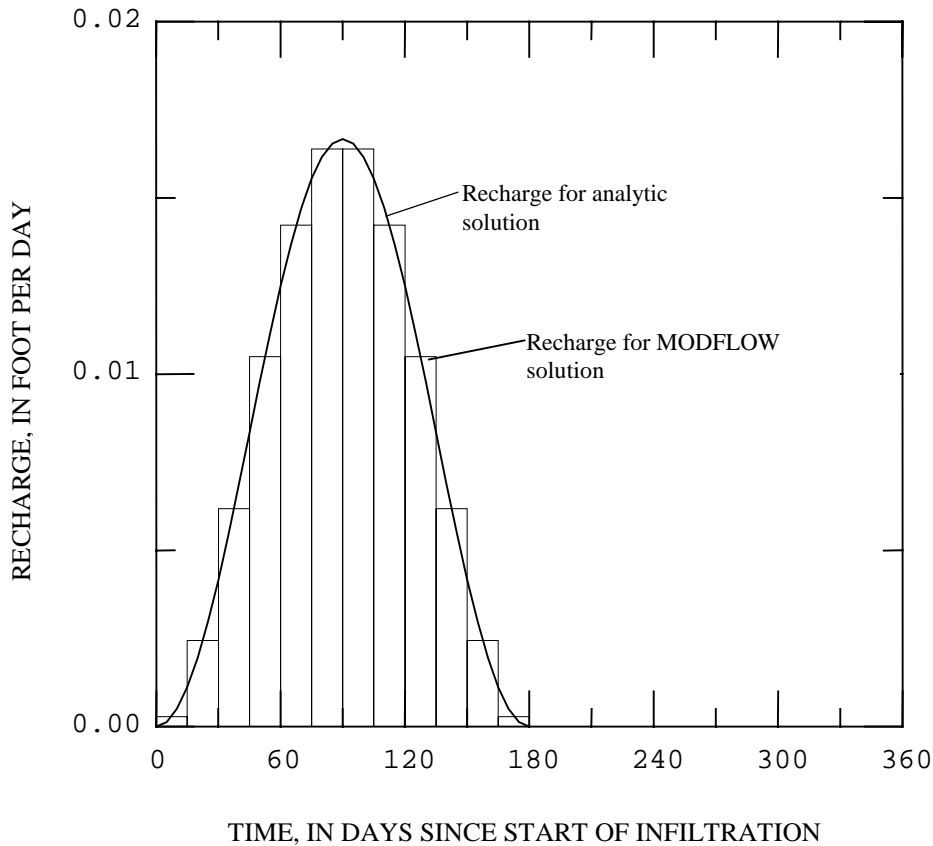
Figure 9. Distribution of recharge used for the analytical and numerical simulation of example 1.
