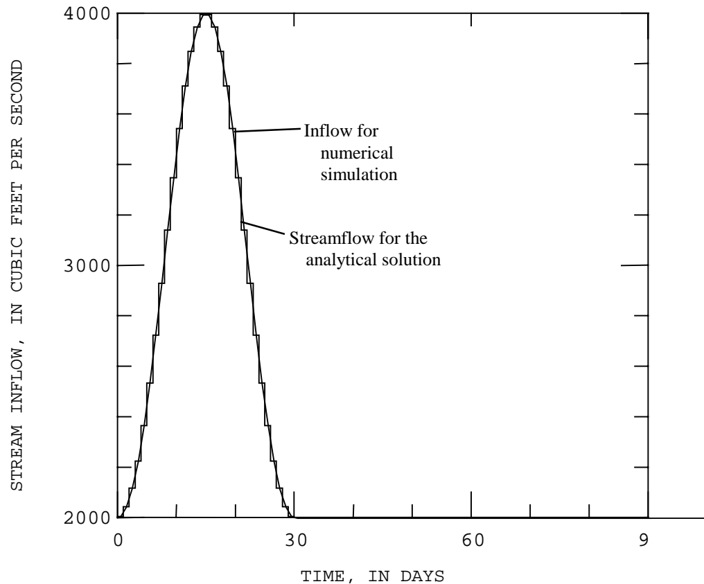
Figure 16. Distribution of streamflow for a 30-day flood event used in example 2.
