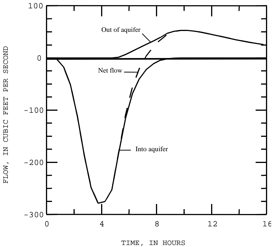
Figure 25. Flow into and out of the aquifer of example 3 as a function of time.
