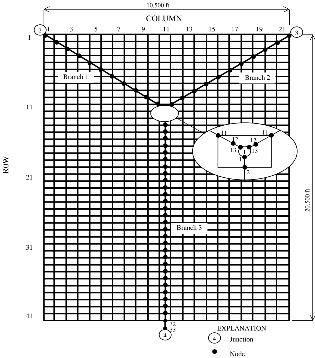
Figure 20. Ground-water model grid of example 3 with surface-water model grid superimposed.
