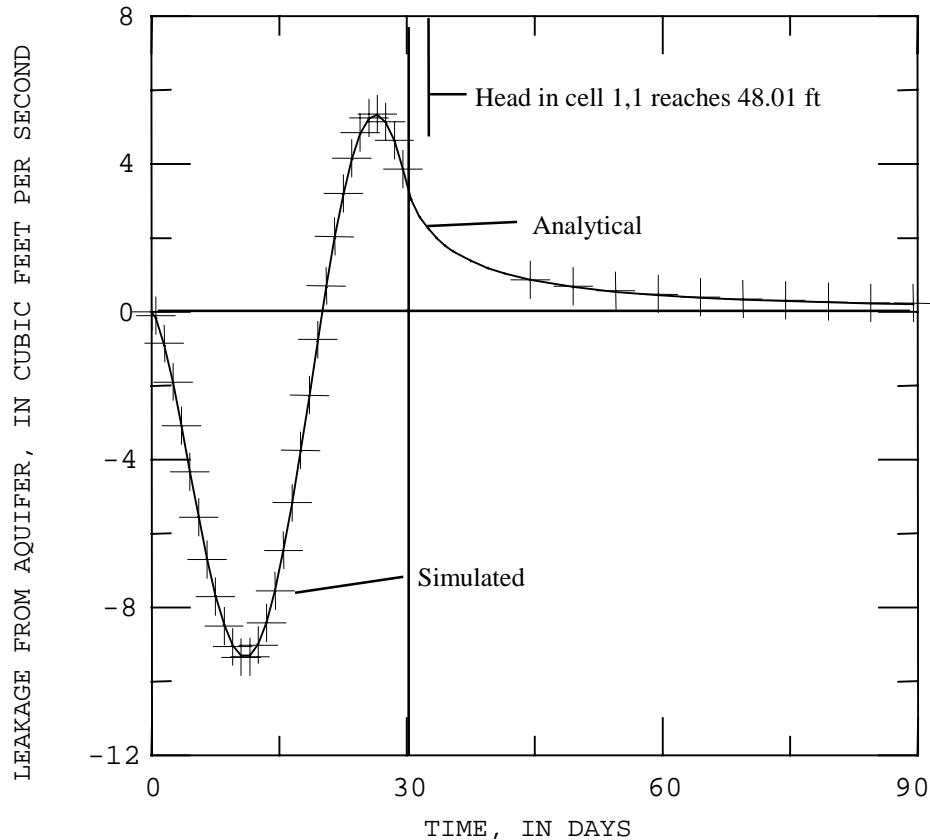
Figure 19. Simulated and analytical flow between the aquifer and the stream for example 2.
