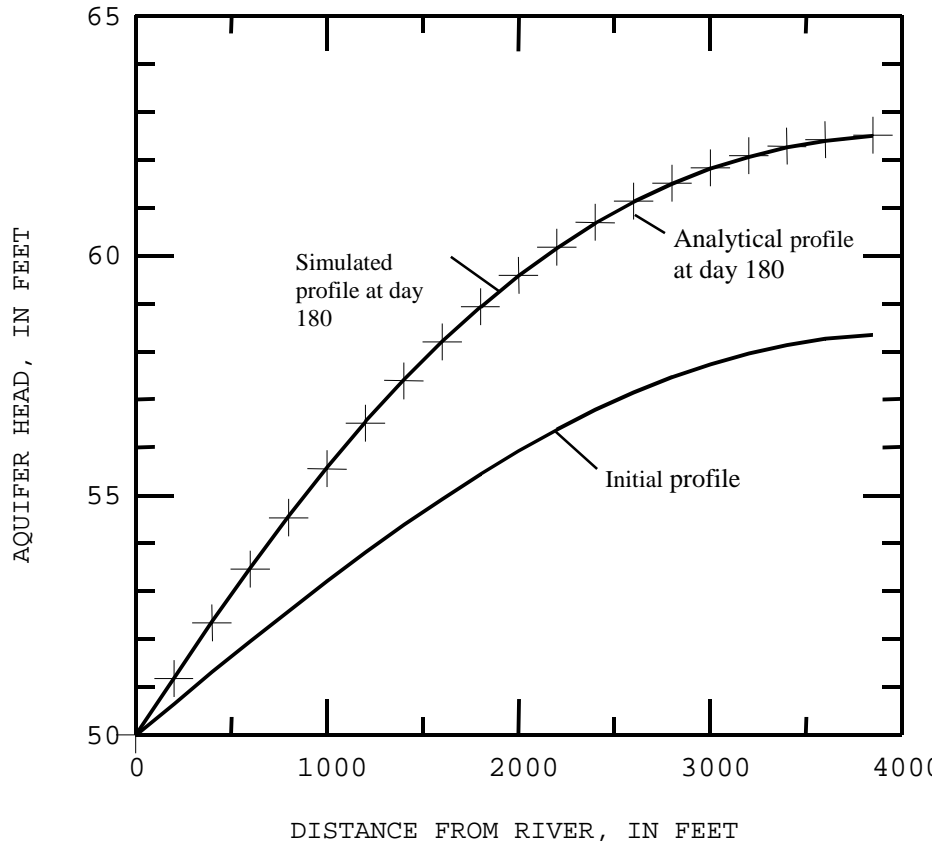
Figure 15. Aquifer-head profiles simulated by the Diffusion Analogy Flow model linked to the Modular Finite-Difference Ground-Water Flow model and the analytical solution.
