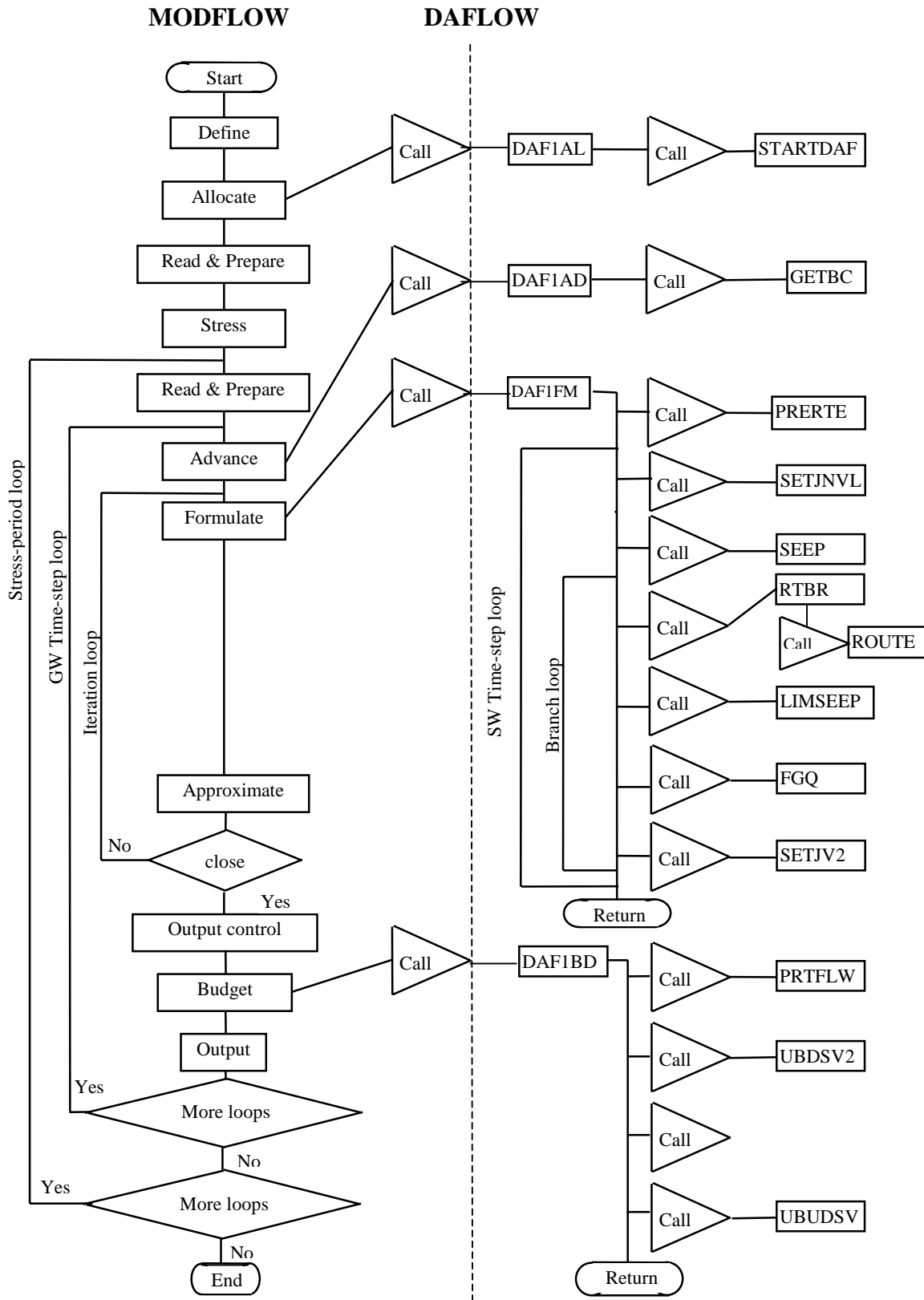
Figure 5. Overall program structure of the Diffusion Analogy Flow model linked to the Modular Finite-Difference Ground-Water Flow model.
