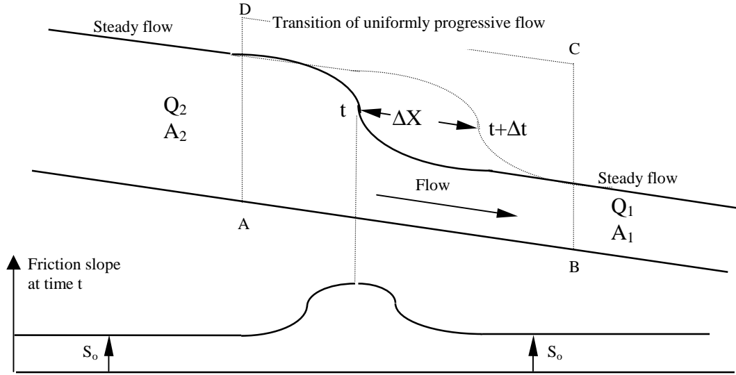
Figure 1. Schematic showing steady uniform flow subreaches connected by a transition of uniformly progressive flow.
