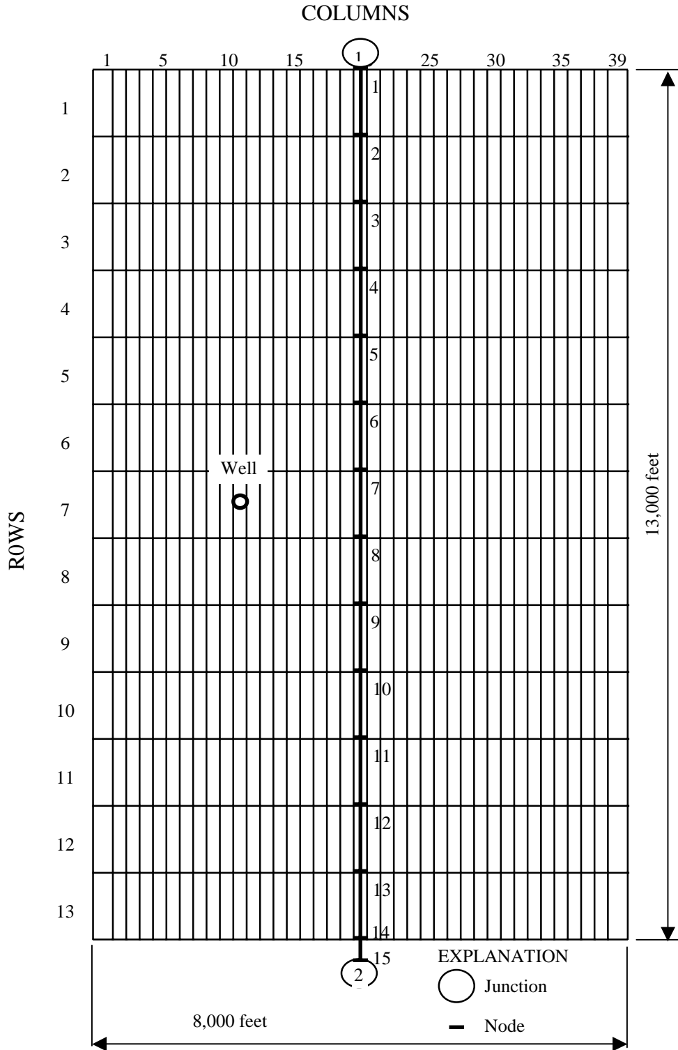
Figure 8. Aquifer grid of example 1 with surface-water model grid superimposed.
