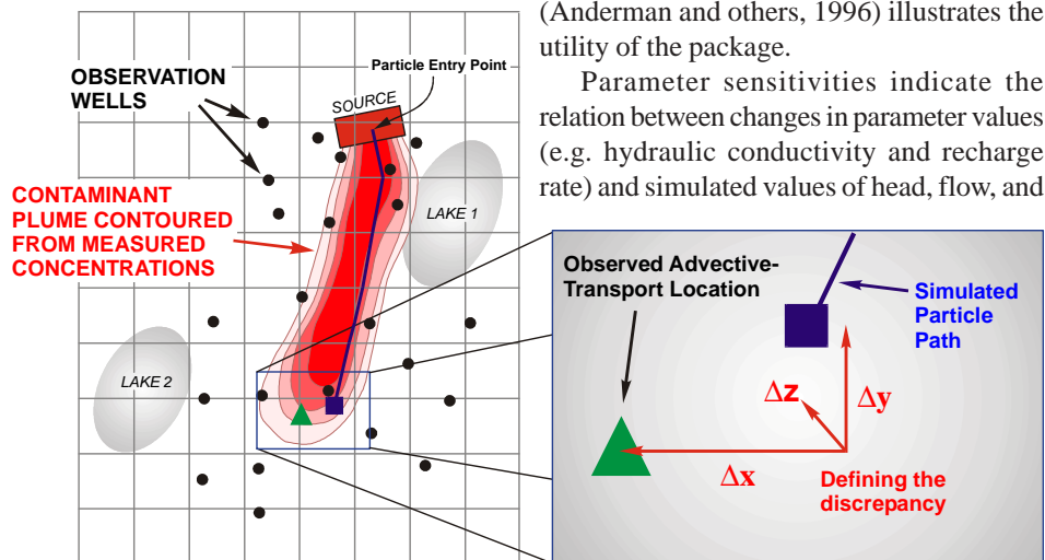
Figure 1. Conceptual representation of advective-transport observations.
