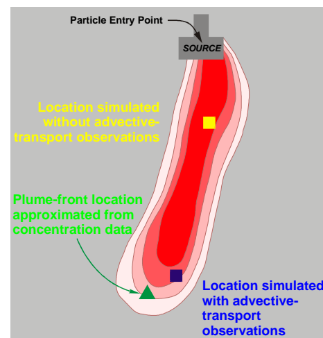
Figure 4. Improved simulated plume movement using advective-transport observations.
