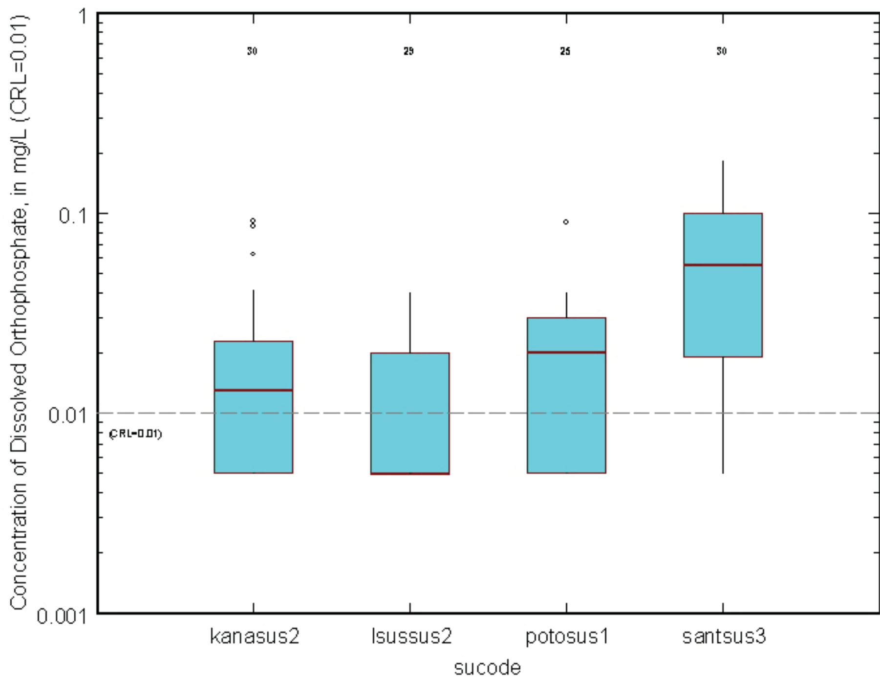
Piedmont and Blue Ridge Crystalline-Rock Aquifers, sus, orthophosphate, number is number of samples
