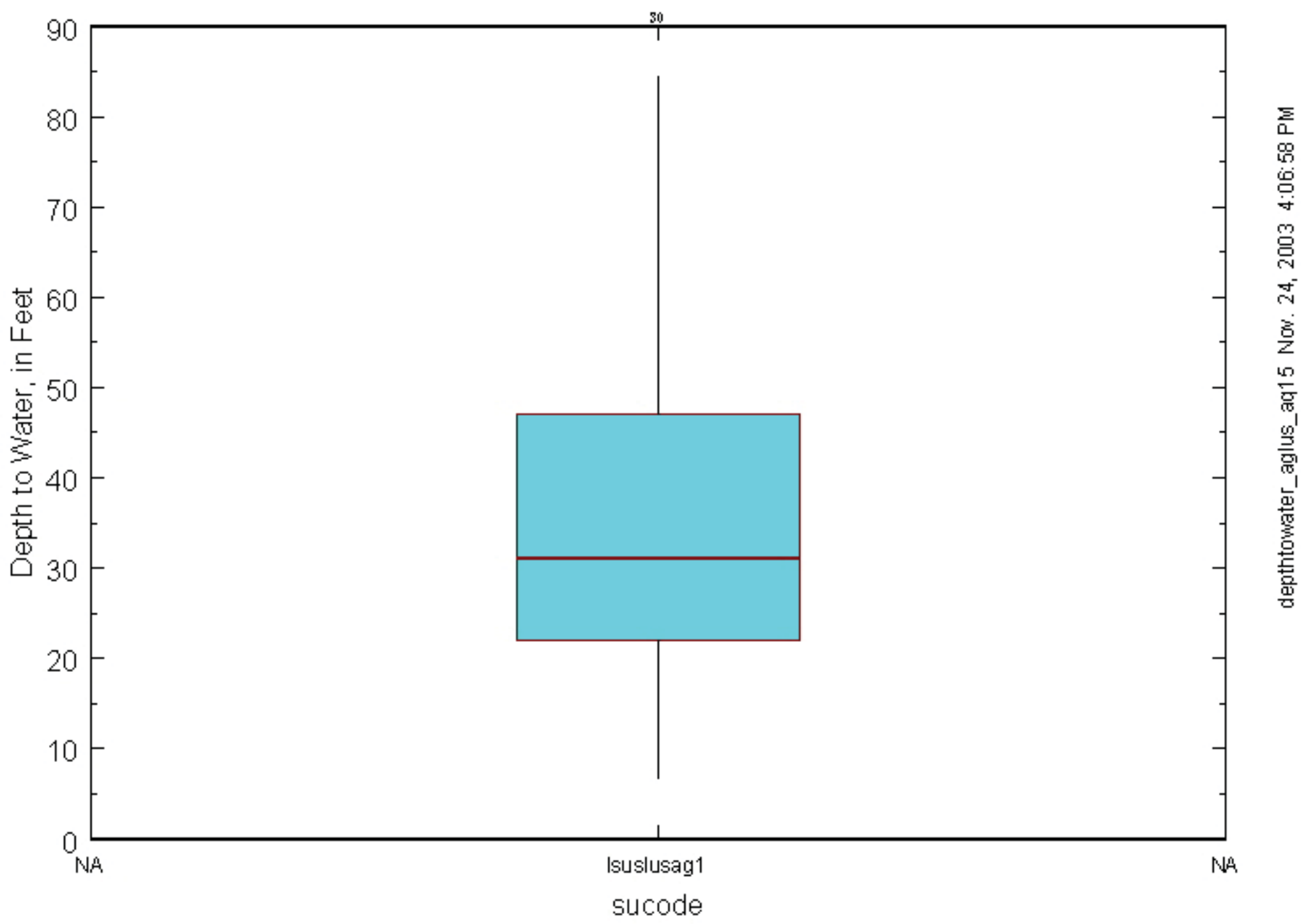
Piedmont and Blue Ridge Carbonate-Rock Aquifers, aglus, depth to water, number is number of samples
