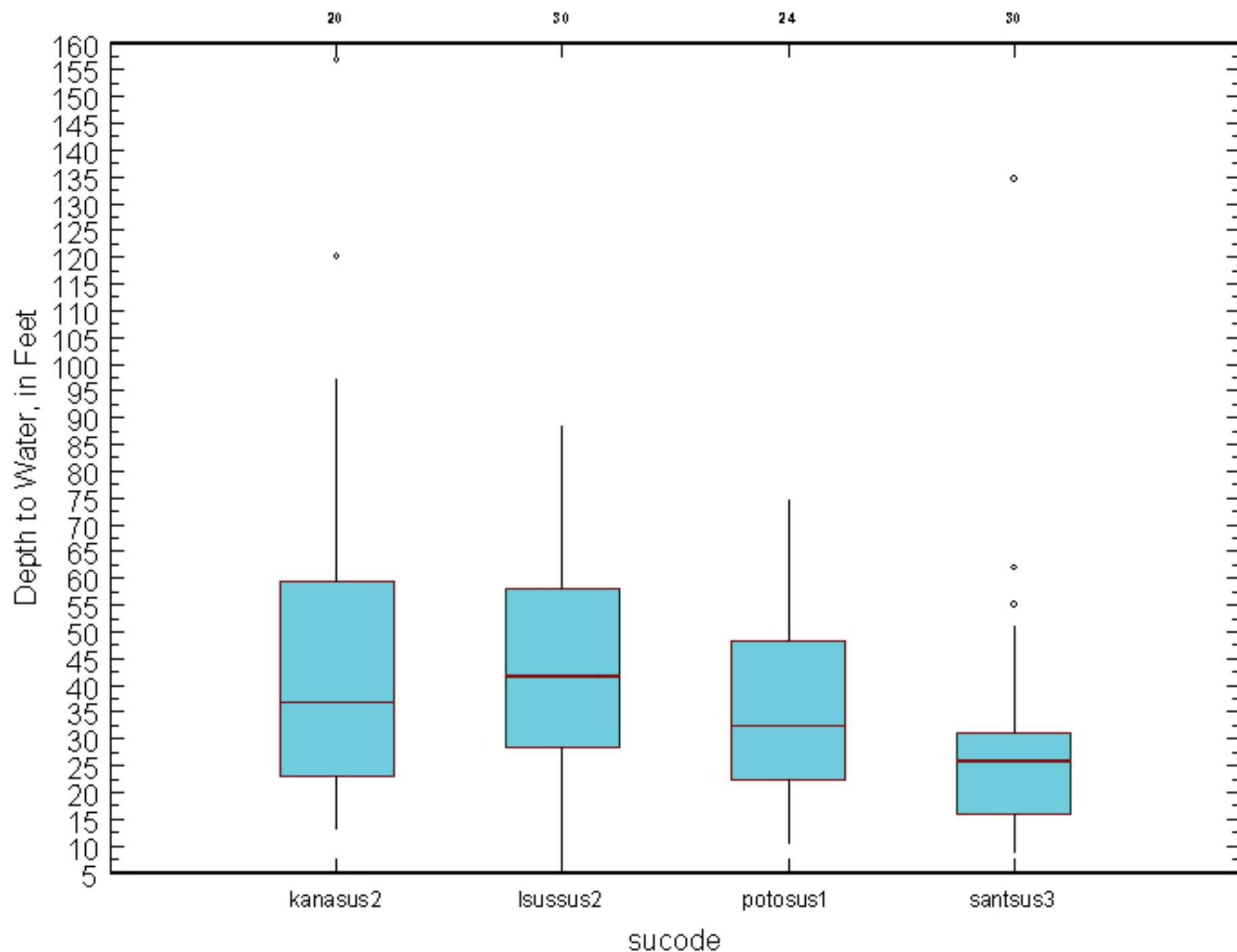
Piedmont and Blue Ridge Crystalline-Rock Aquifers, sus, depth to water, number is number of samples
