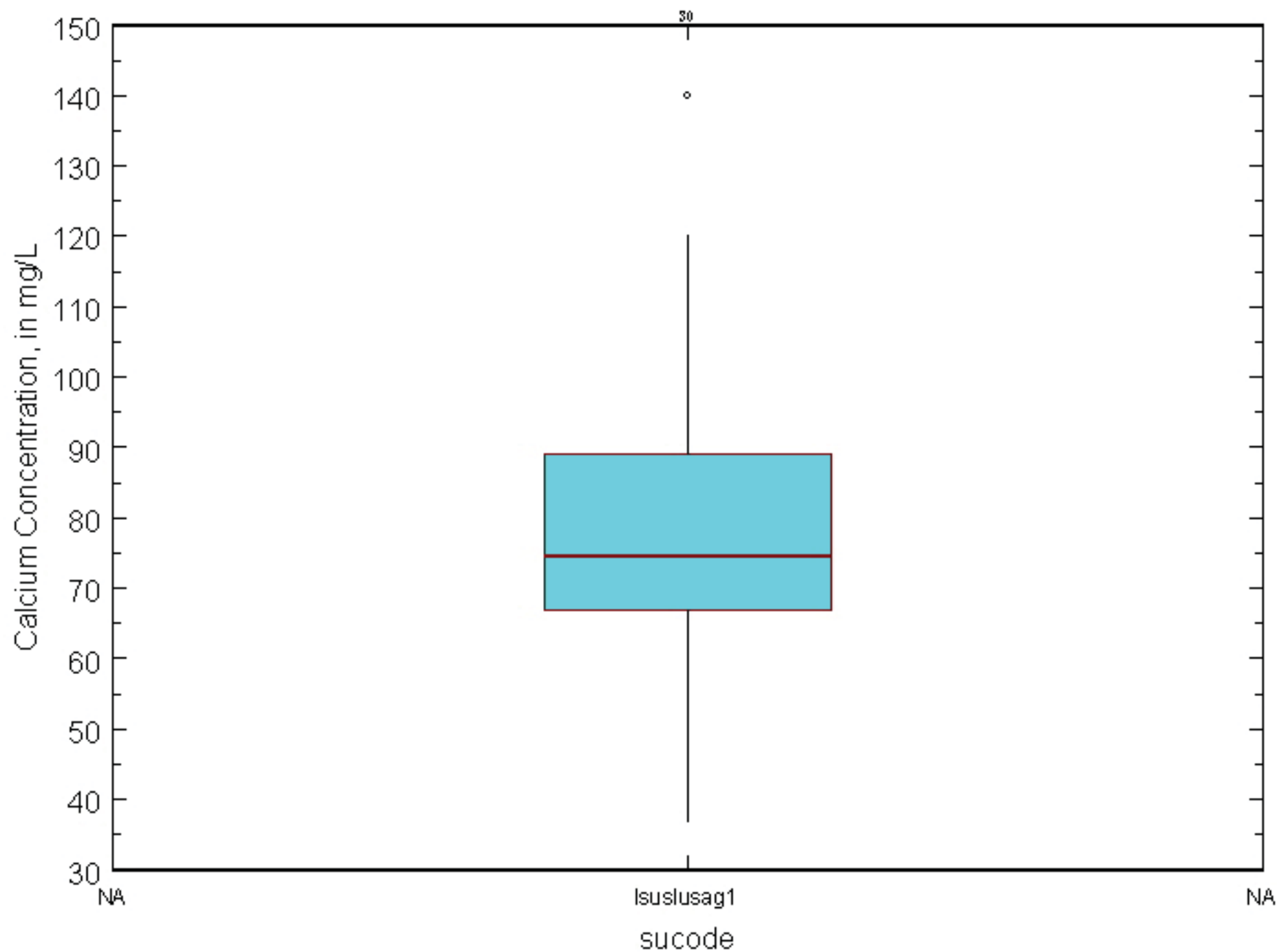
Piedmont and Blue Ridge Carbonate-Rock Aquifers, aglus, calcium, number is number of samples
