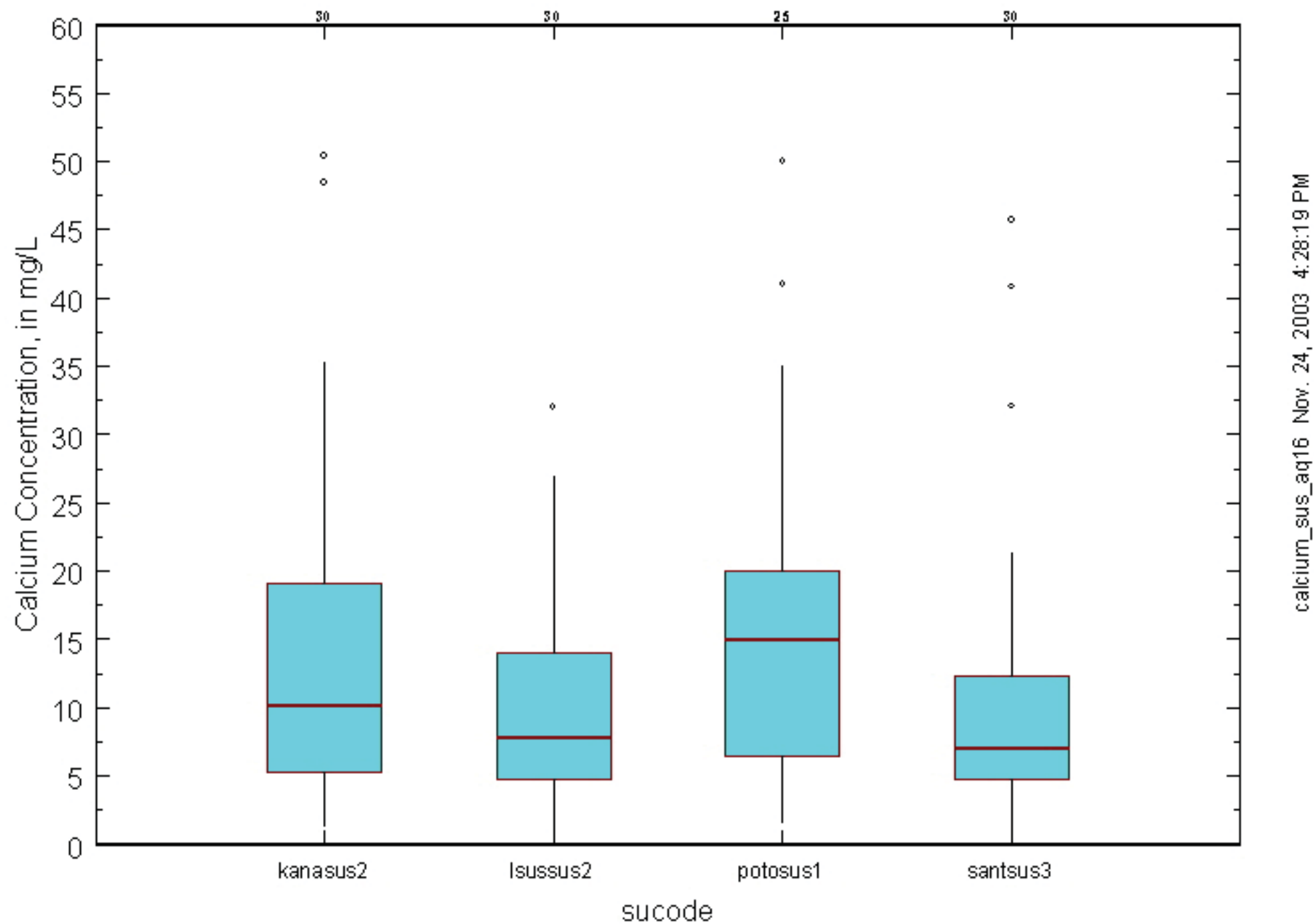
Piedmont and Blue Ridge Crystalline-Rock Aquifers, sus, calcium, number is number of samples
