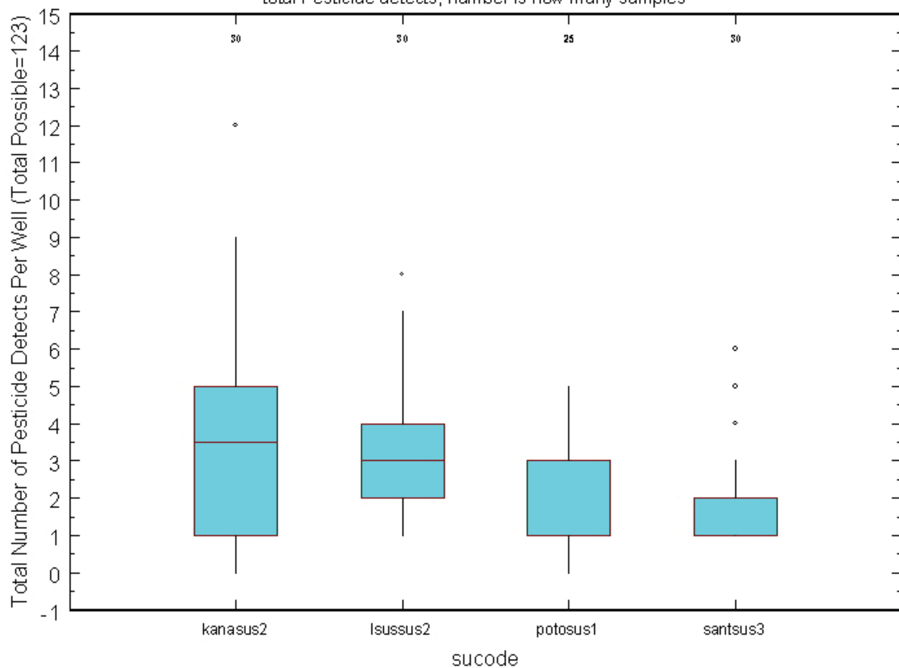
Piedmont and Blue Ridge Crystalline-Rock Aquifers, sus, total Pesticide detects, number is how many samples
