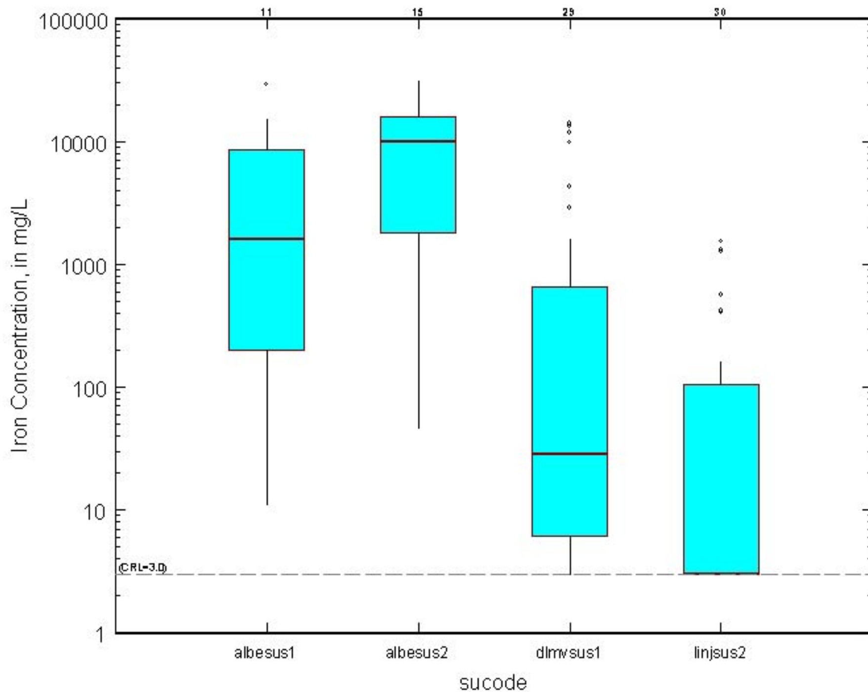
North Atlantic Coastal Plain Aquifer System, sus, iron, number is number of samples
