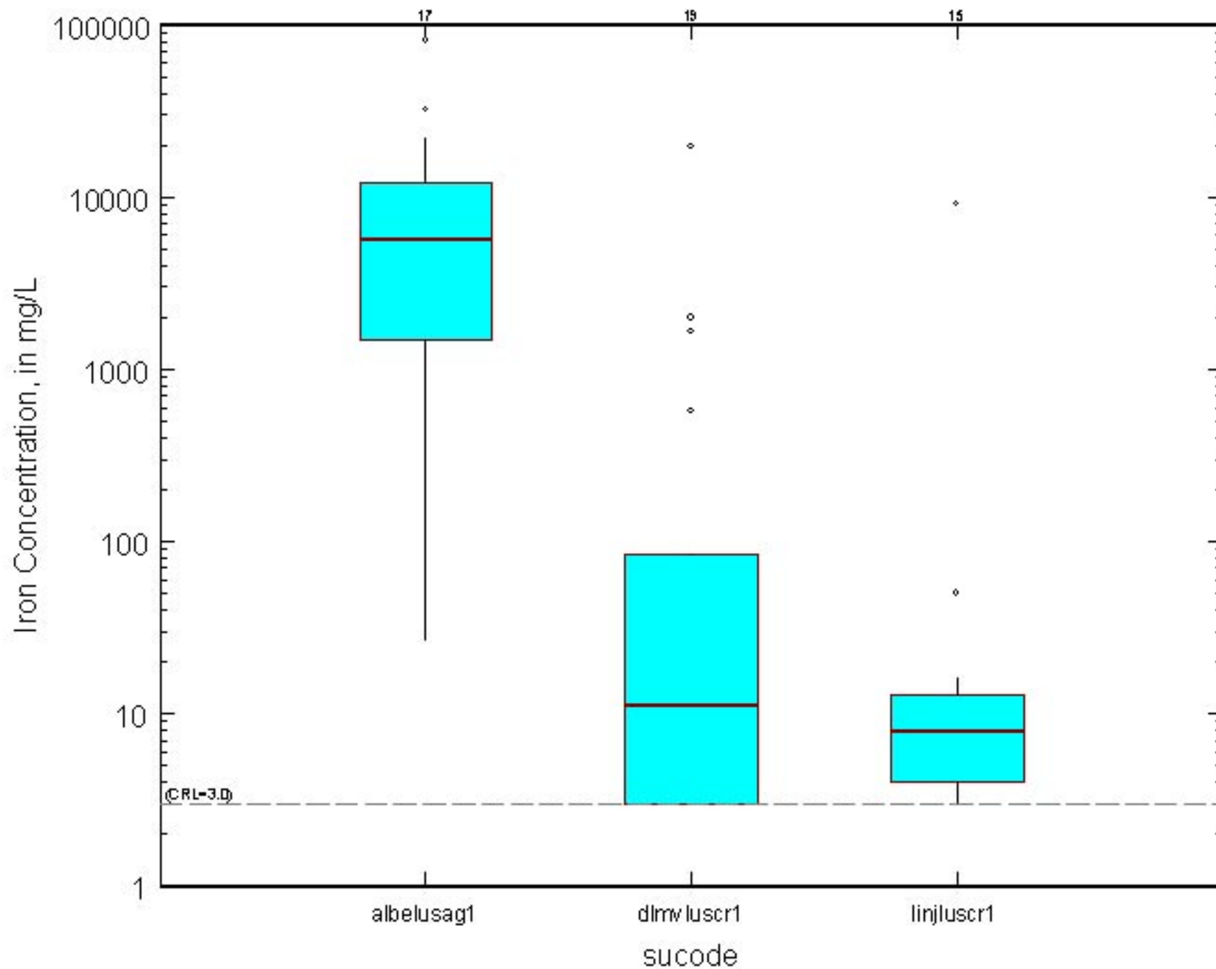
North Atlantic Coastal Plain Aquifer System, aglus, iron, number is number of samples
