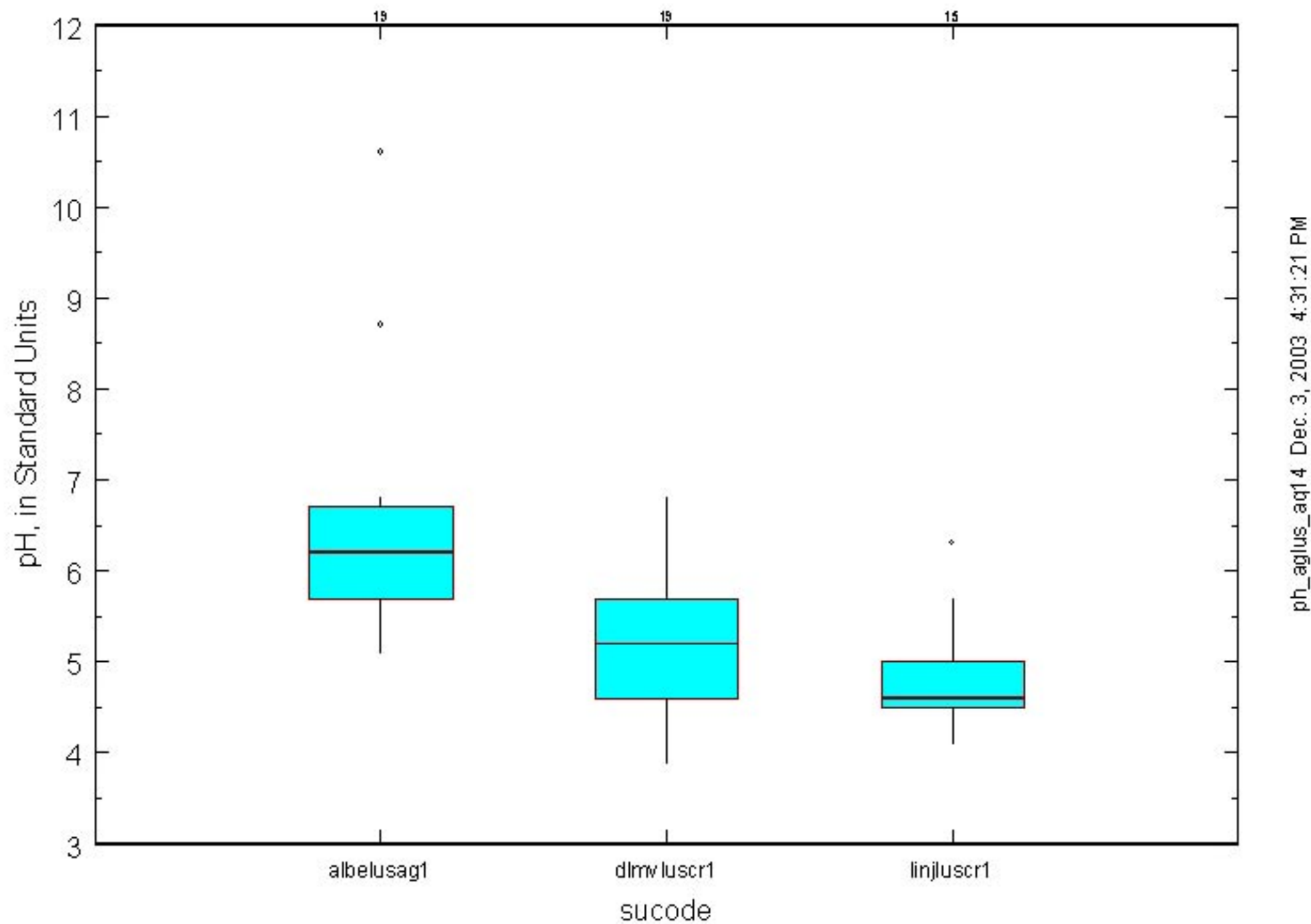
North Atlantic Coastal Plain Aquifer System, aglus, pH, number is number of samples
