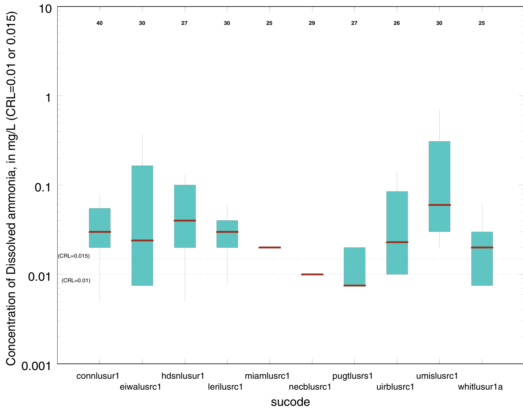
Glacial-deposit Aquifers, urblus, ammonia, number is number of samples
