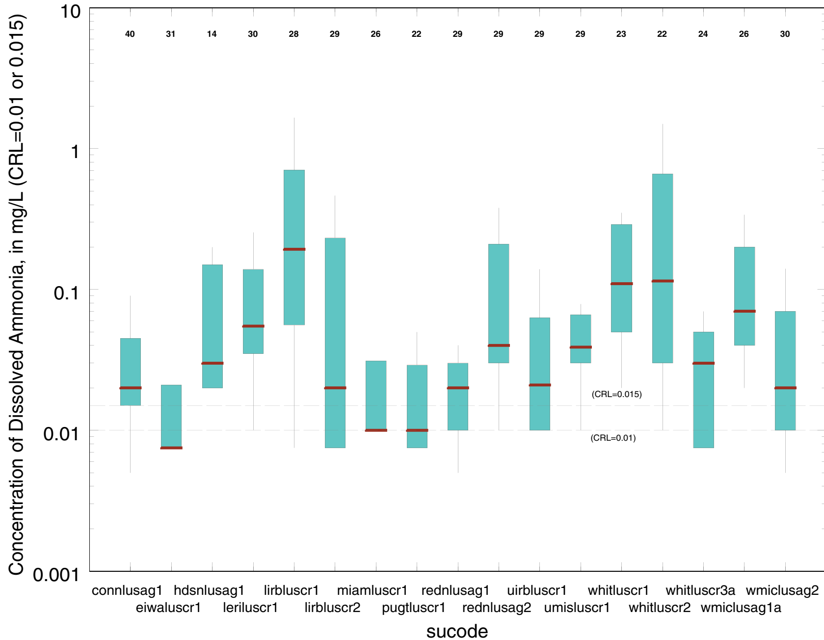
Glacial-deposit Aquifer, aglus, ammonia, number is number of samples
