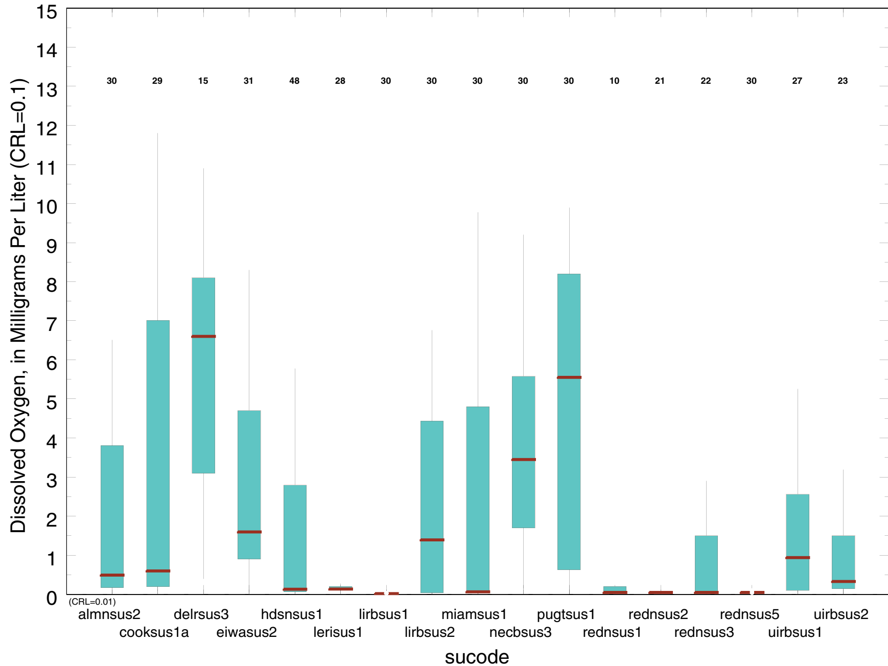
Glacial-deposit Aquifers, sus, dissolved oxygen, number is number of samples
