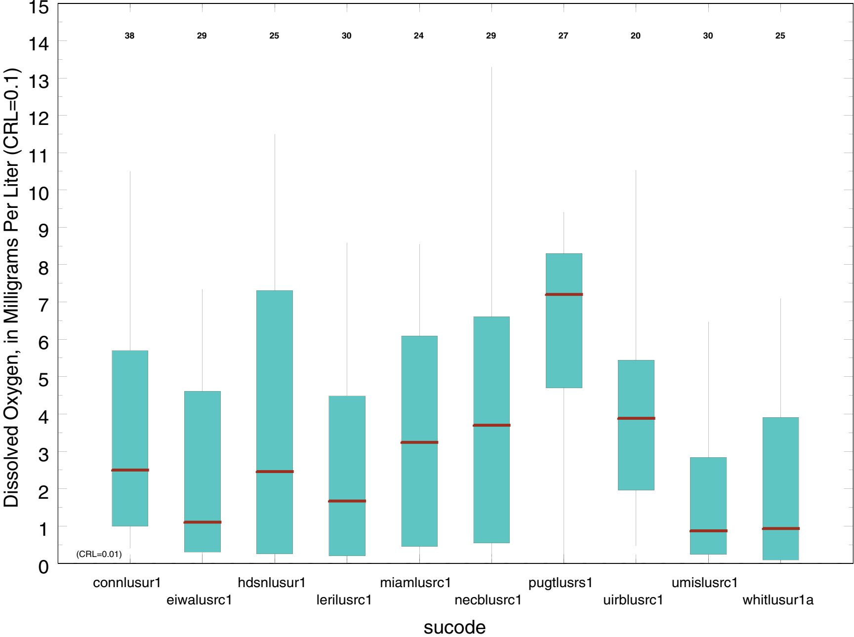
Glacial-deposit Aquifers, urblus, dissolved oxygen, number is number of samples
