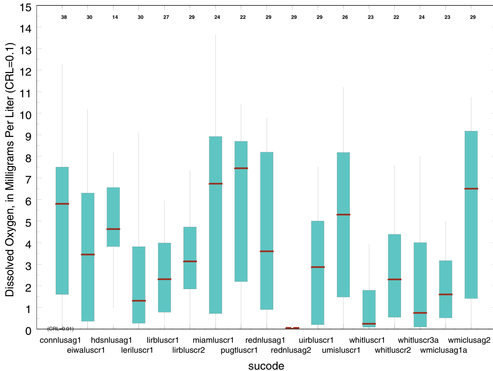
Glacial-deposit Aquifers, aglus, dissolved oxygen, number is number of samples
