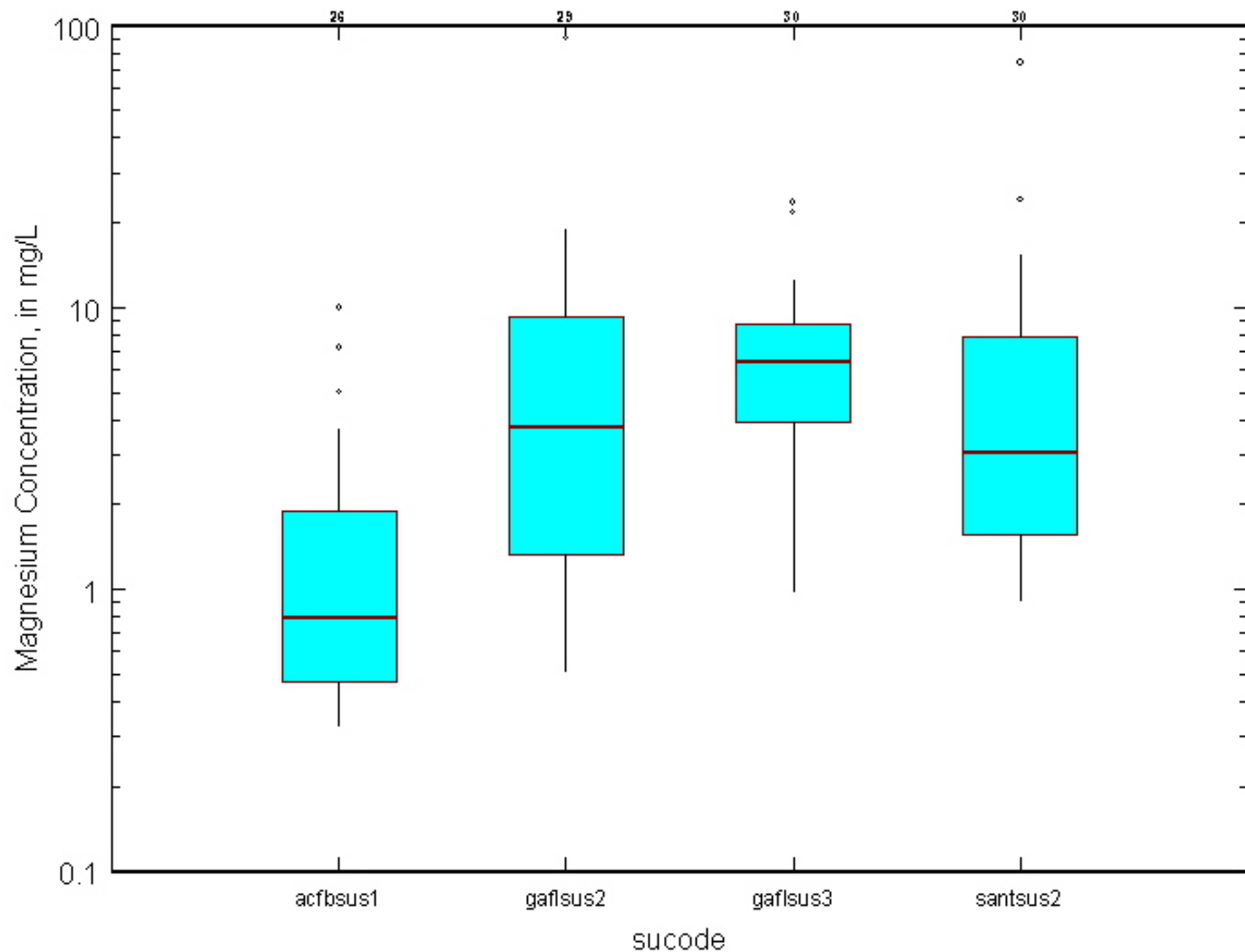
Floridan Aquifer System, sus, magnesium, number is number of samples
