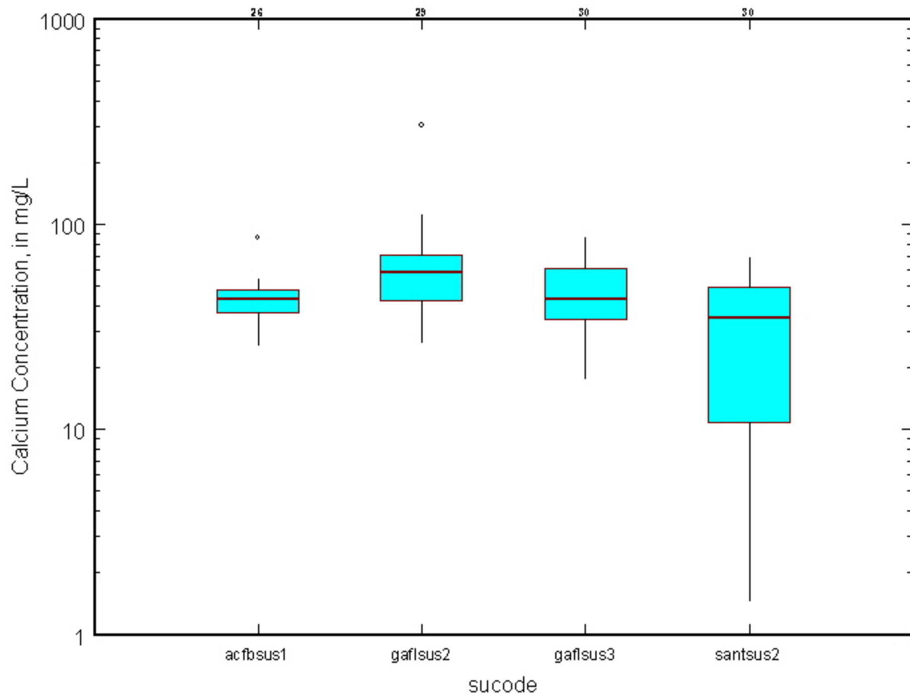
Floridan Aquifer System, sus, calcium, number is number of samples
