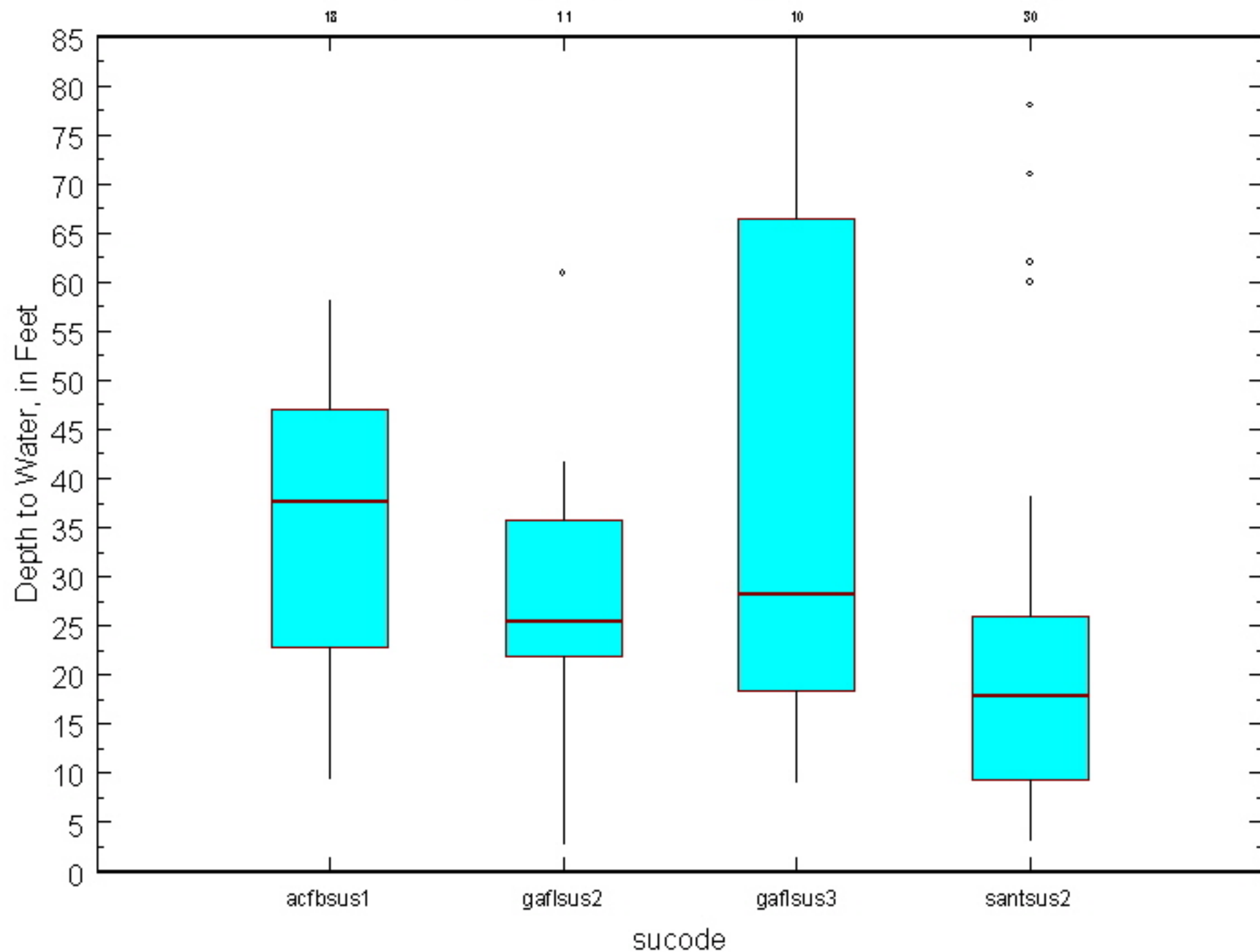
Floridan Aquifer System, sus, depth to water, number is number of samples
