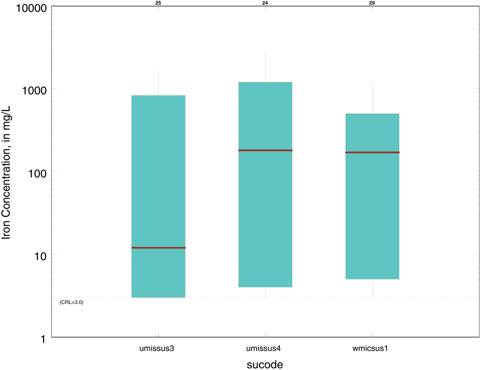
Cambrian-Ordovician Aquifer System, sus, iron, number is number of samples
