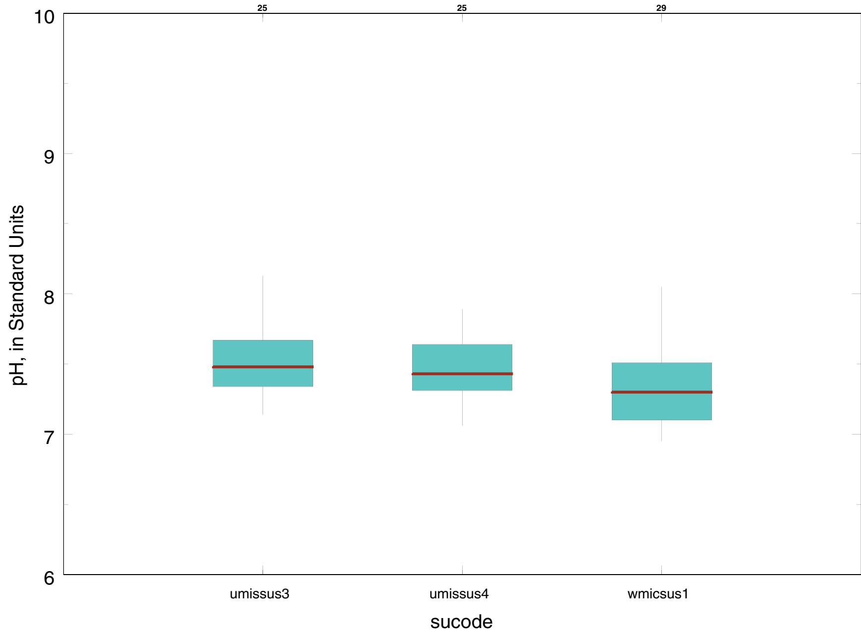
Cambrian-Ordovician Aquifer System, sus, pH, number is number of samples
