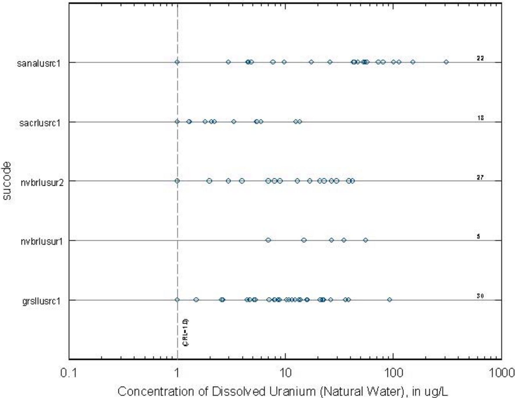
Basin and Range Aquifers (including California Coastal Basin and Central Valley), urblus, uranium (CRL=1.0 ug/L)
