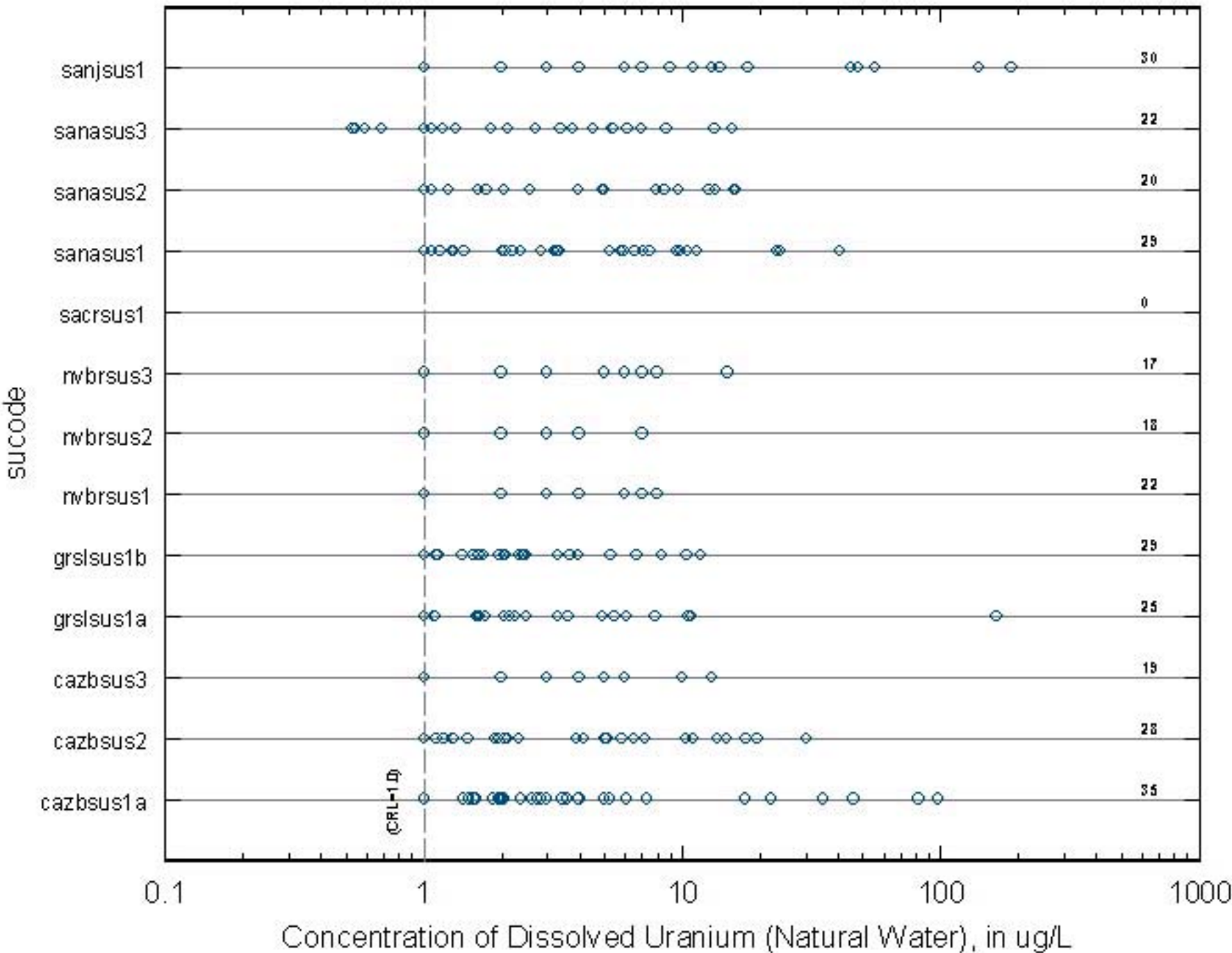
Basin and Range Aquifers (including California Coastal Basin and Central Valley), sus, uranium (CRL=1.0 ug/L)
