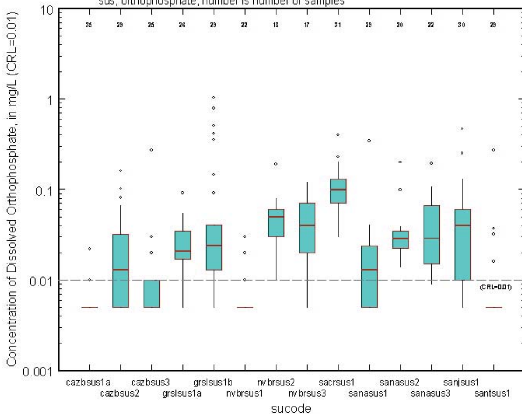
Basin and Range Aquifers (including California Coastal Basin and Central Valley), sus, orthophosphate, number is number of samples
