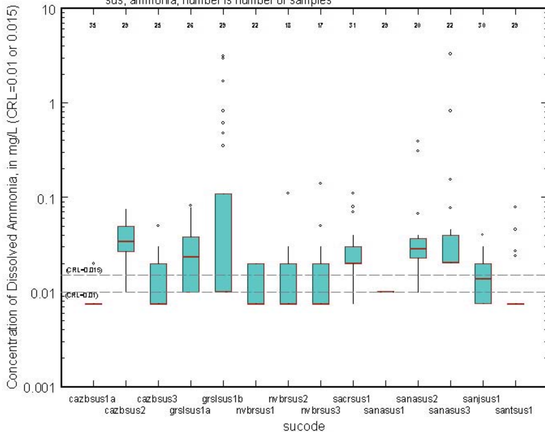
Basin and Range Aquifers (including California Coastal Basin and Central Valley), sus, ammonia, number is number of samples
