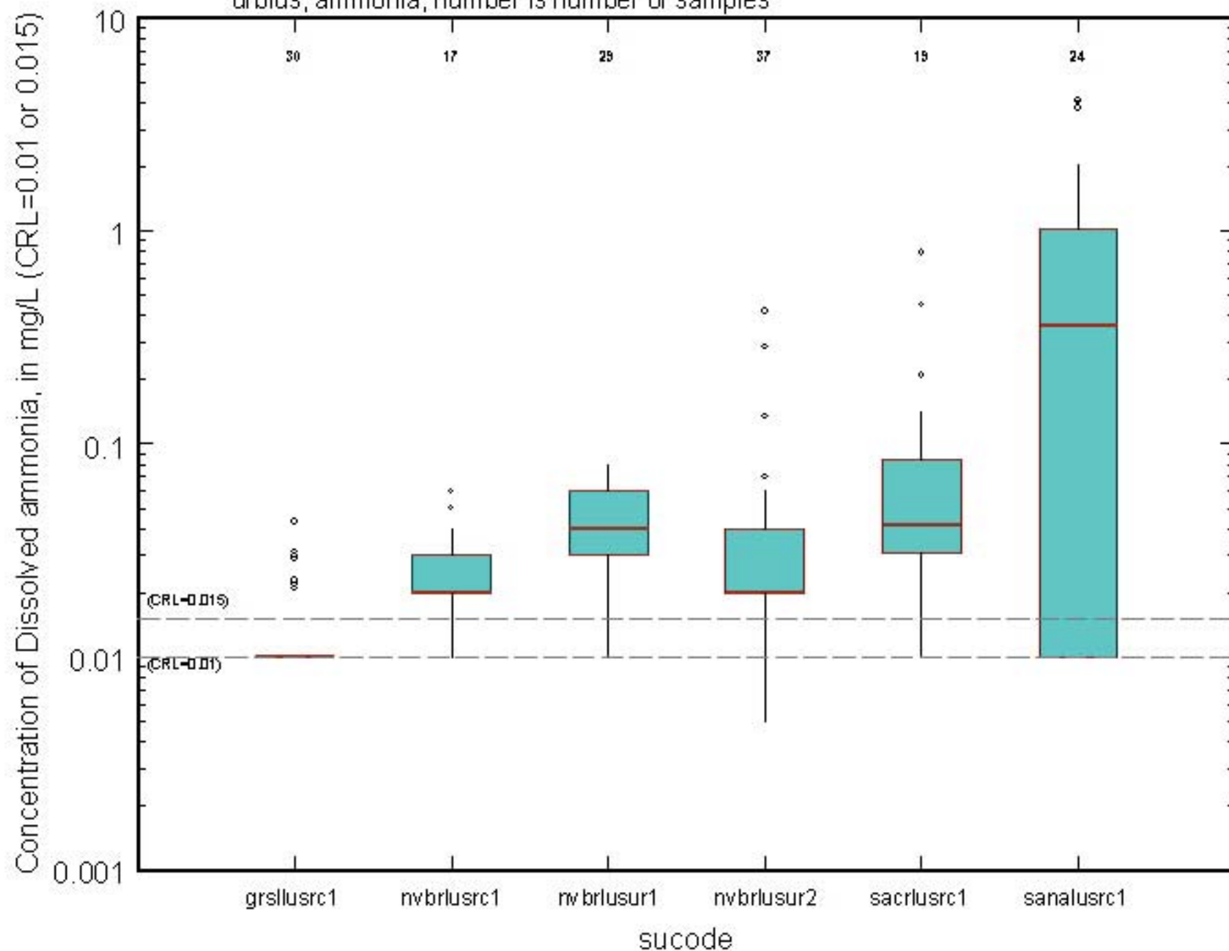
Basin and Range Aquifers (including California Coastal Basin and Central Valley), urblus, ammonia, number is number of samples
