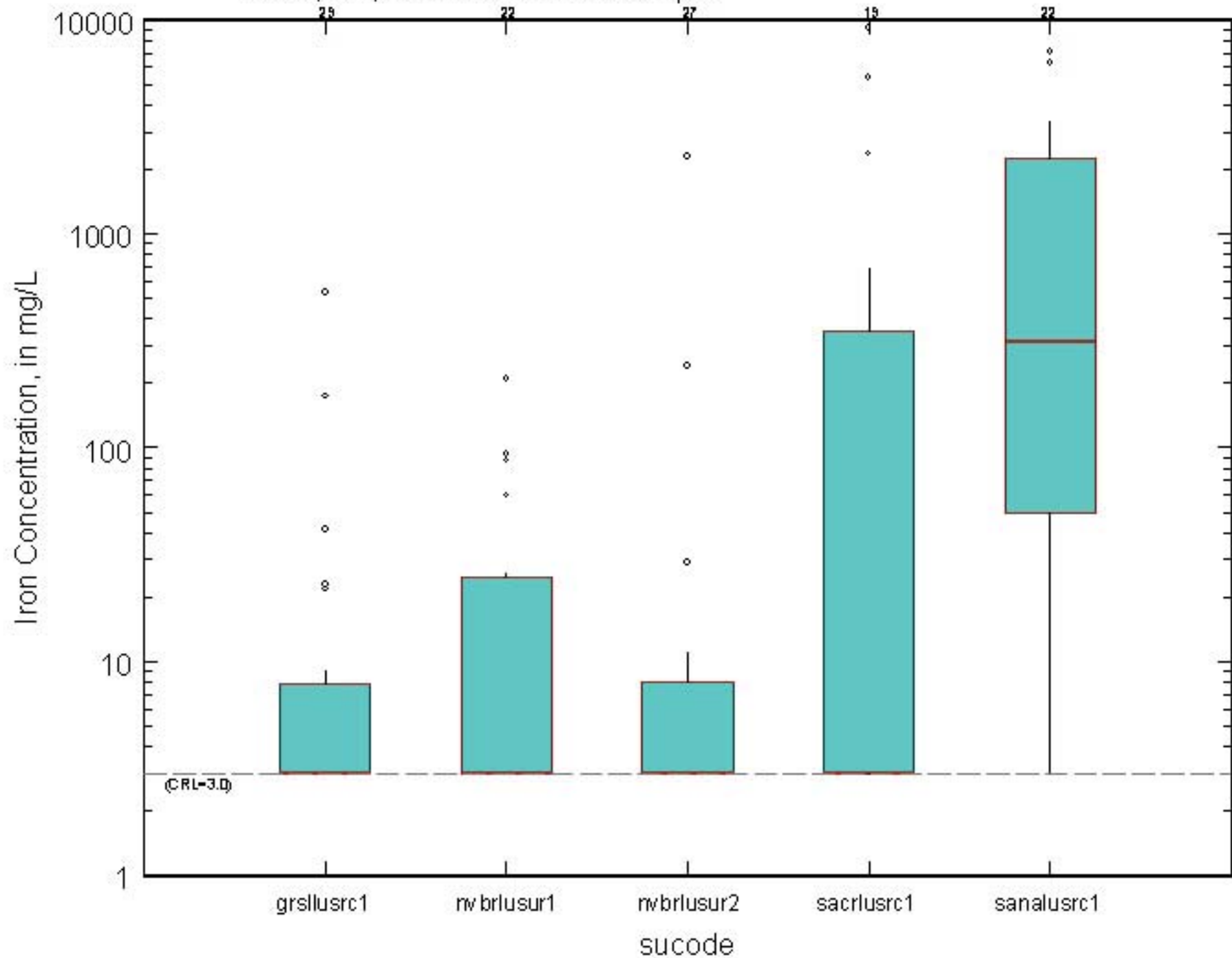
Basin and Range Aquifers (including California Coastal Basin and Central Valley), urblus, iron, number is number of samples
