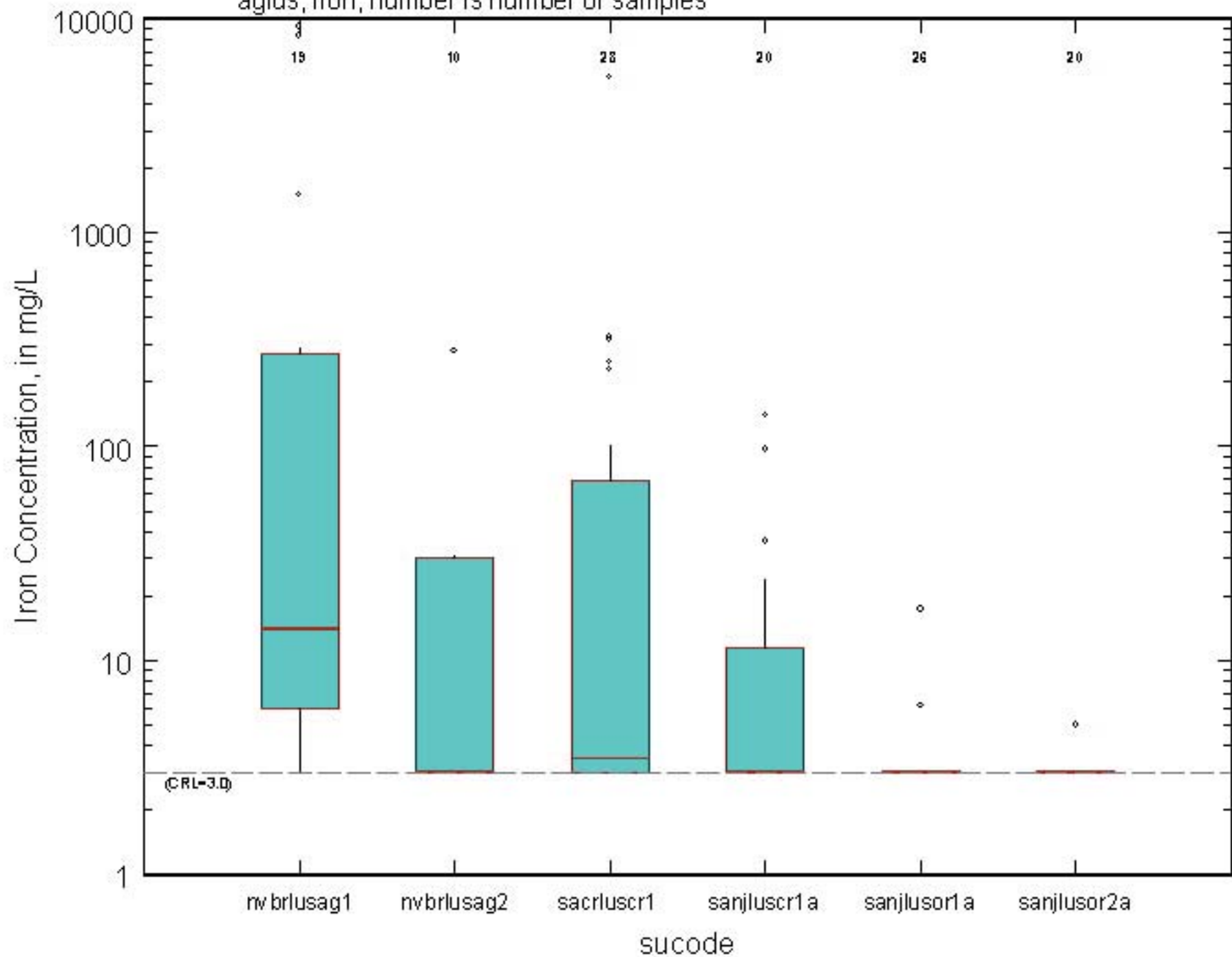
Basin and Range Aquifers (including California Coastal Basin and Central Valley), aglus, iron, number is number of samples
