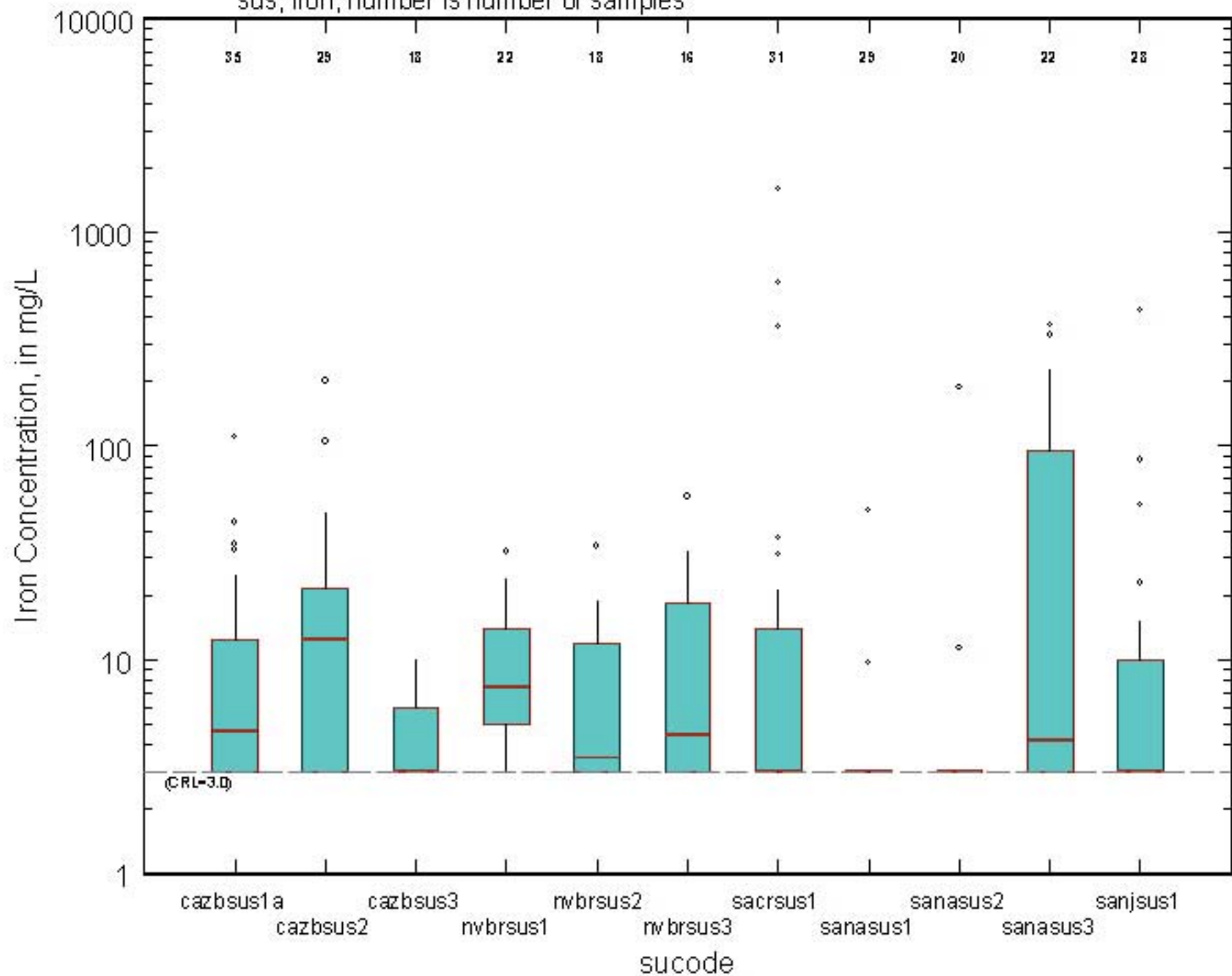
Basin and Range Aquifers (including California Coastal Basin and Central Valley), sus, iron, number is number of samples
