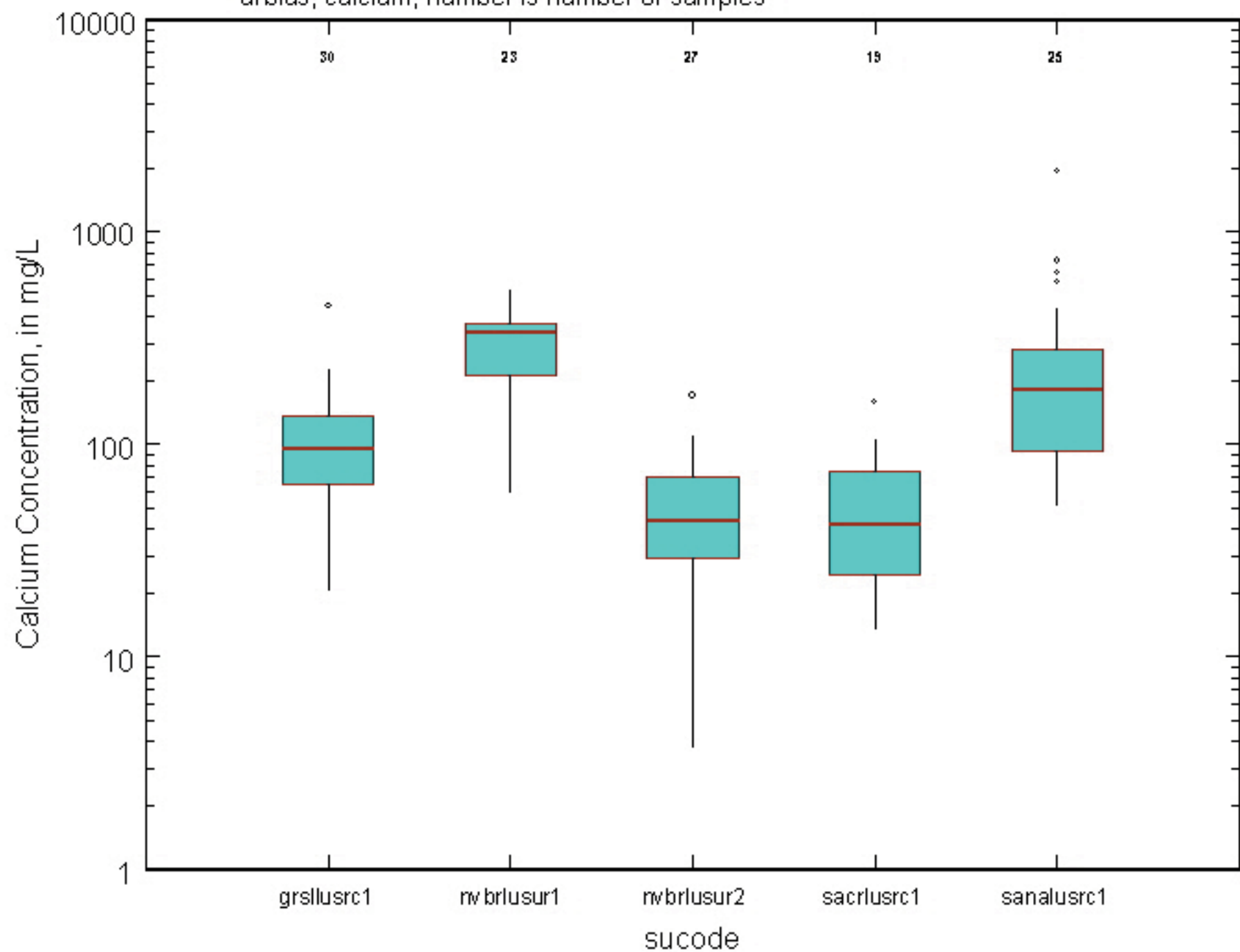
Basin and Range Aquifers (including California Coastal Basin and Central Valley), urblus, calcium, number is number of samples
