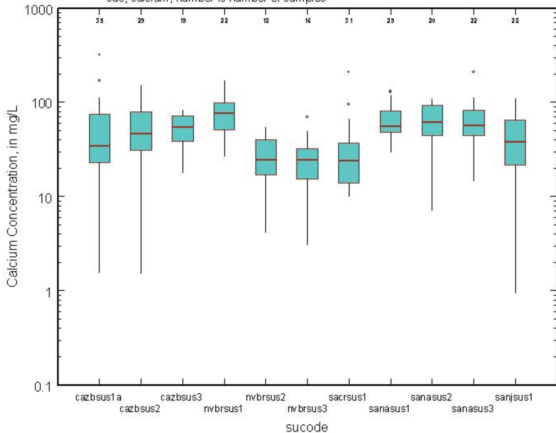
Basin and Range Aquifers (including California Coastal Basin and Central Valley), sus, calcium, number is number of samples
