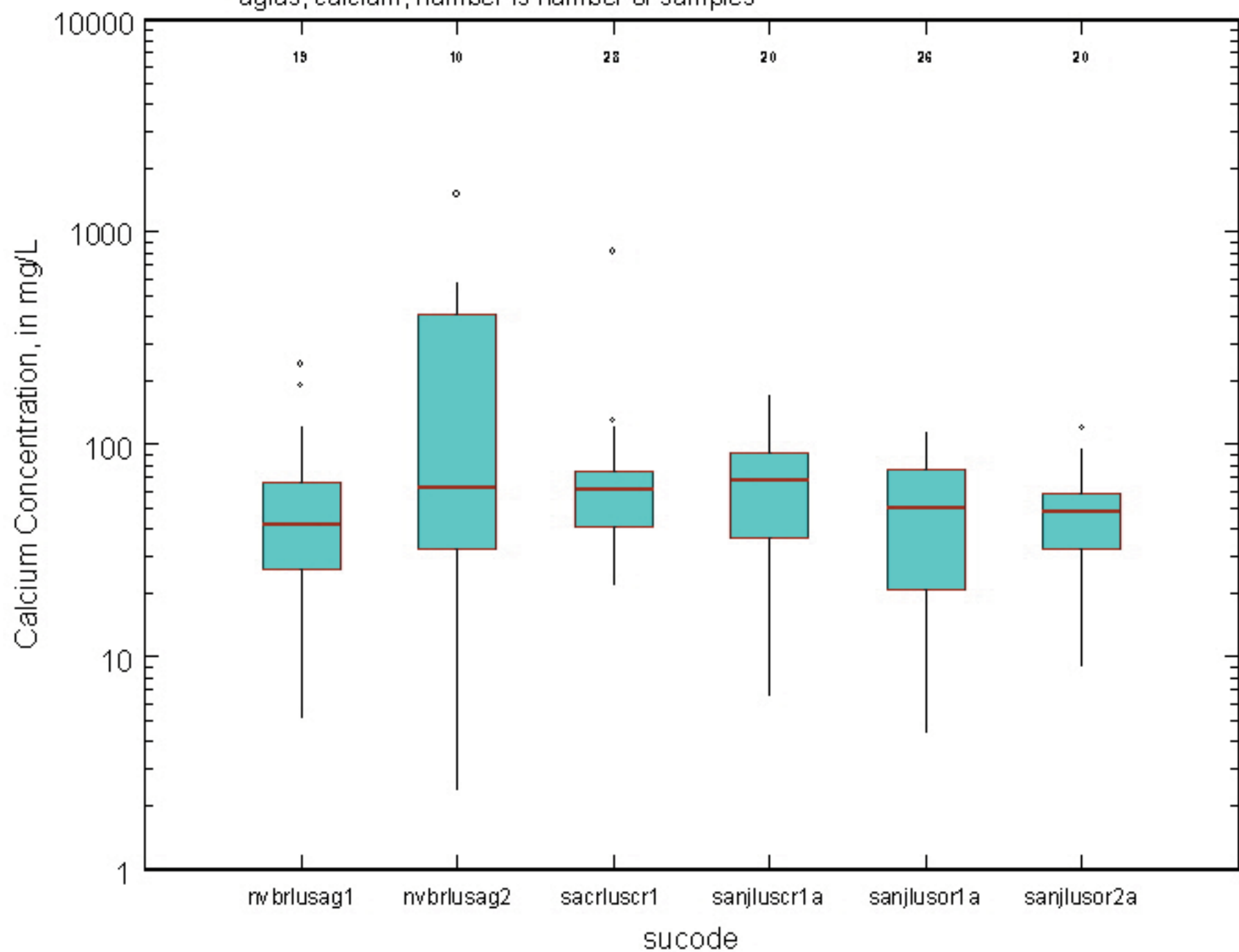
Basin and Range Aquifers (including California Coastal Basin and Central Valley), aglus, calcium, number is number of samples
