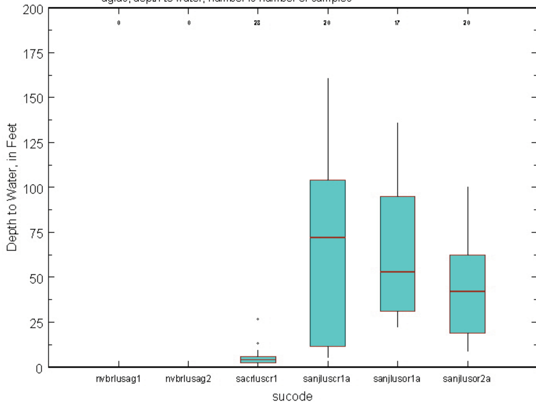
Basin and Range Aquifers (including California Coastal Basin and Central Valley), aglus, depth to water, number is number of samples
