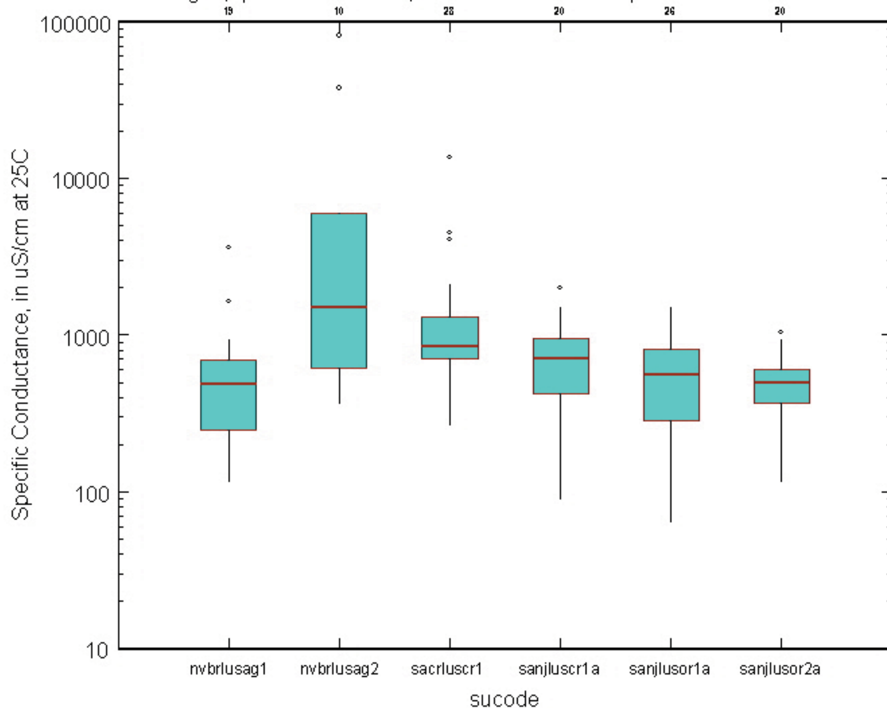
Basin and Range Aquifers (including California Coastal Basin and Central Valley), aglus, specific conductance, number is number of samples
