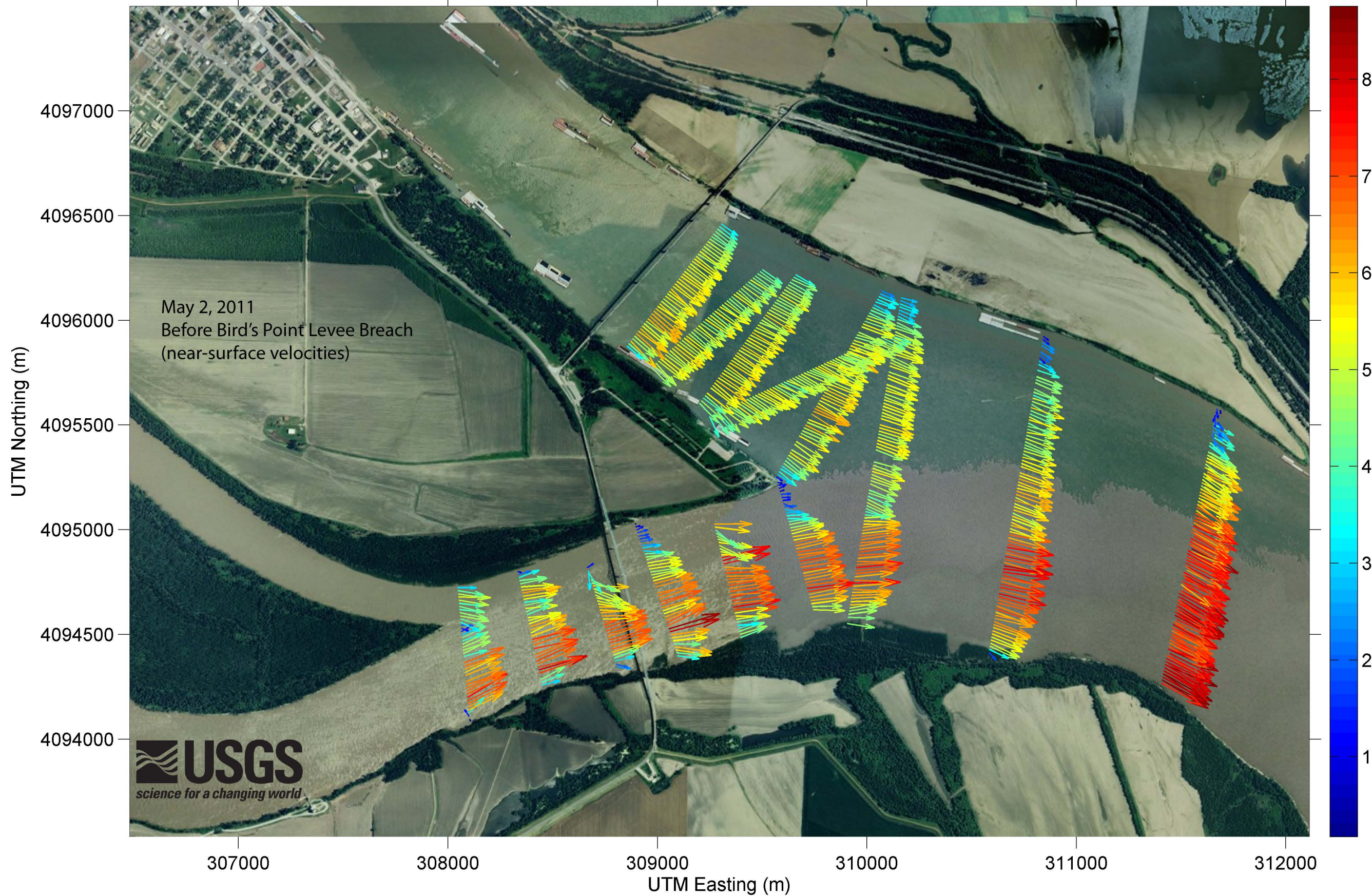
Depth-Averaged Velocities (ft/s) Averaged over depths 0ft to 6.562ft
