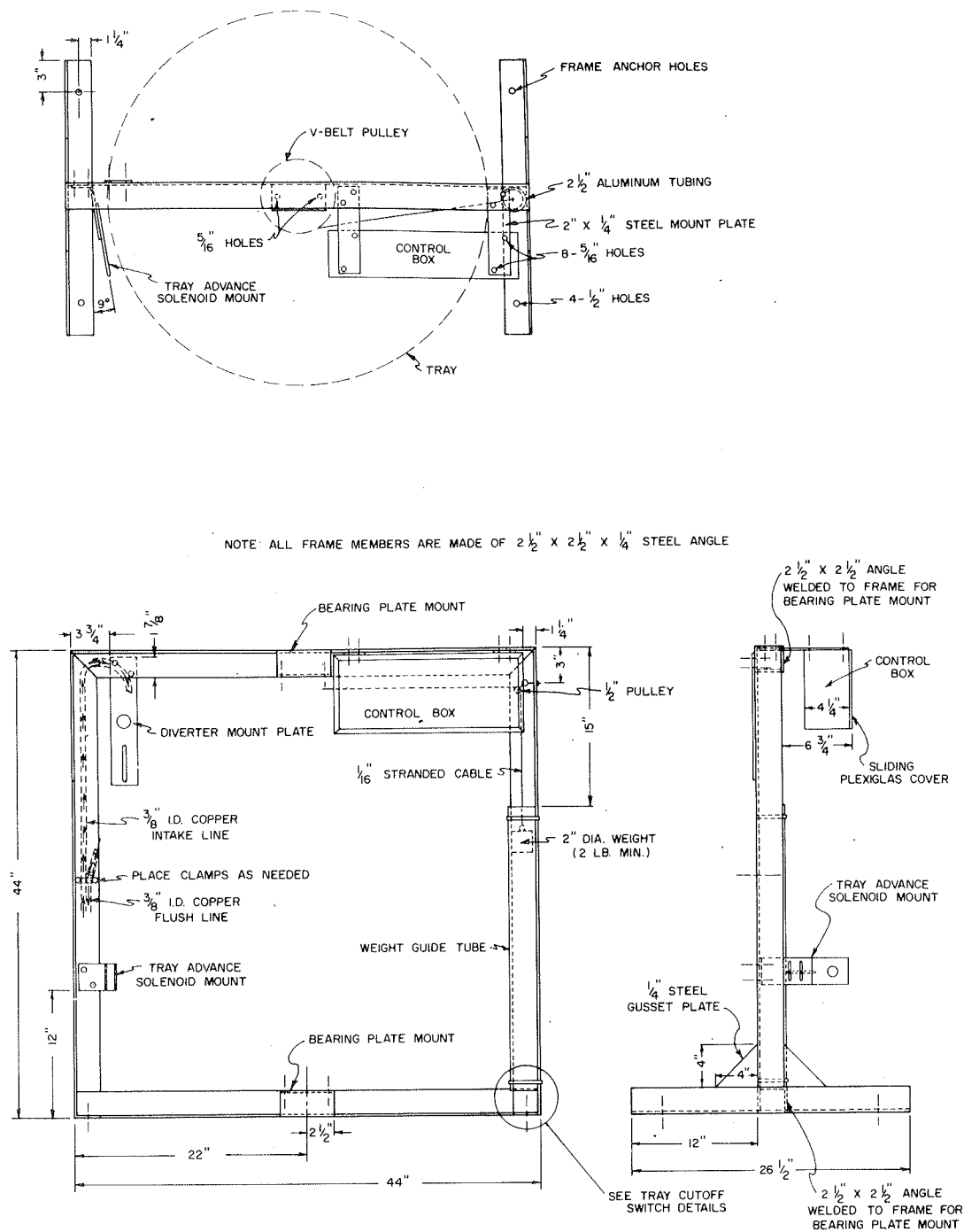
FIGURE 4.—Frame assembly with details.
