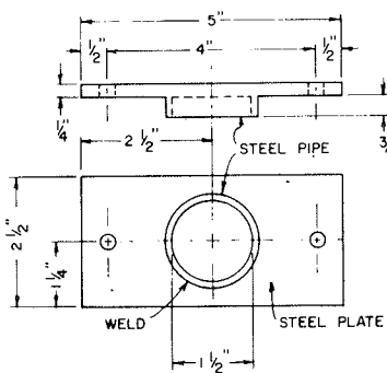
UPPER BEARING PLATE
