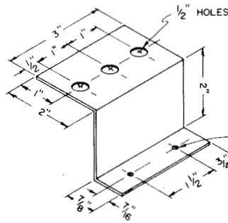
BRACKET 1
