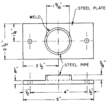
LOWER BEARING PLATE
