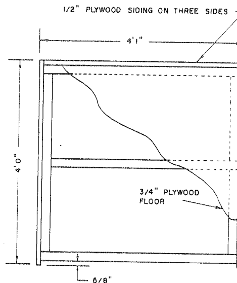
FLOOR DETAIL
