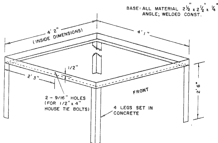
BASE DETAIL
