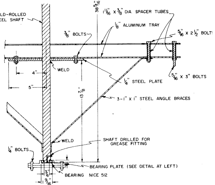
TRAY ASSEMBLY DETAILS
