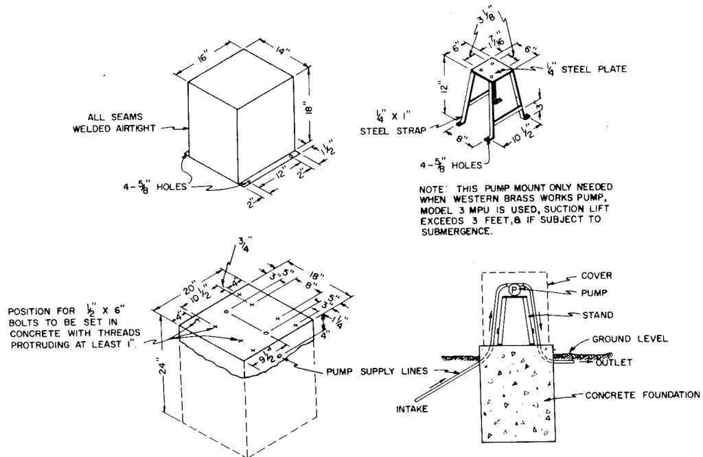
FIGURE 3.—Details of tray cutoff switch and stationary pump mount.
