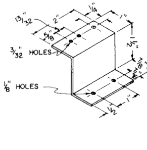
BRACKET 2
