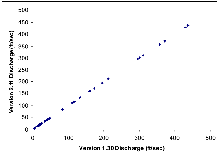
Figure A-1. Comparison of 40 discharge measurements computed, using version 1.30 and 2.11 FlowTracker Software.
