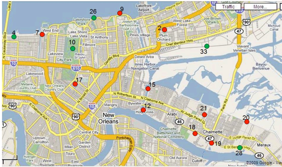
Figure 1b. The map of arsenic distribution in the greater New Orleans area Key: Red dot: > 20 \mu\text{g/L} (ppb); Green dot < 20 \mu\text{g/L} (ppb)
