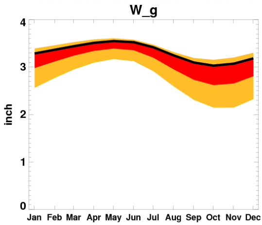
Figure 8. Same as figure 8 except this is for the Canonsville Reservoir in the nearby Catskill Mountains. The time period used for this analysis is 1959-1988.
