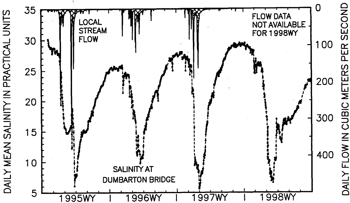
Fig. 8. Daily mean salinity at Dumbarton Bridge and daily mean flow from local streams for water years 1995-1998.
