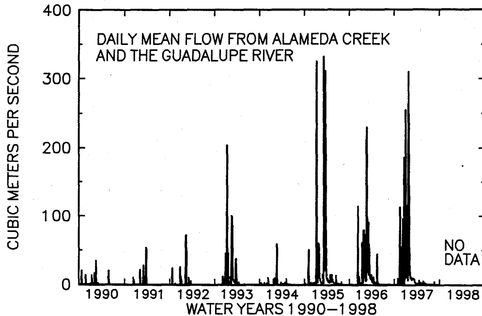
Fig. 5. Total daily mean flow from Alameda Creek and the Guadalupe River to South San Francisco Bay for the 1990-1997 water years. Data are from USGS annual reports for 1990-1997. Data for 1998 were not available when this report was written.
