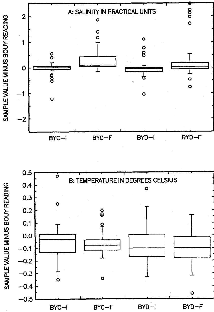
Fig. 7. Differences between recorded values from BYC and BYD and samples collected during deployment (initial, I) and retrieval (final, F). Boxes enclose 50 percent of the values with the median value near the center. The whiskers extending vertically from the boxes are equal to 1.5 times the quartile ranges from the median. Values that lie outside the ranges of the whiskers are shown individually.
