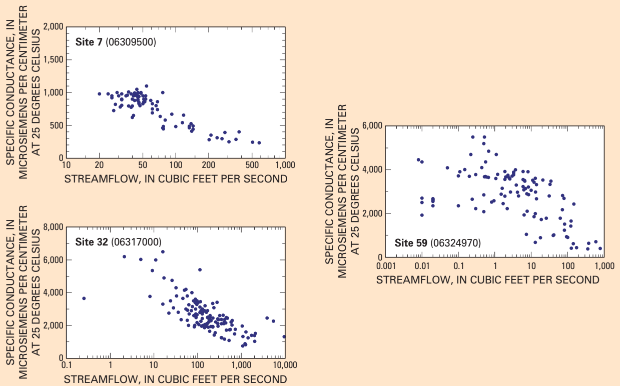
Figure 4. Streamflow and specific-conductance relations at selected sites in the Powder River Basin, Wyoming and Montana.
