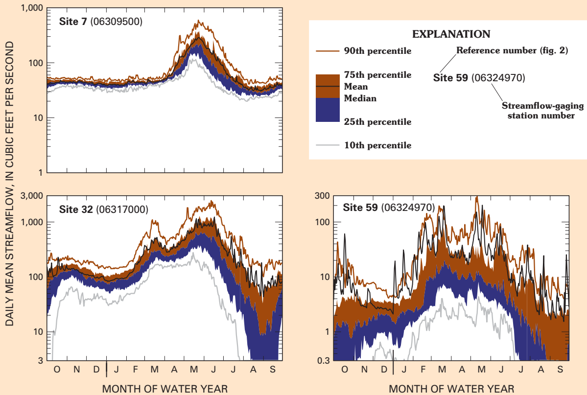
Figure 3. Statistical summary of daily mean streamflow for period of record at selected streamflow-gaging stations, Powder River Basin, Wyoming and Montana.
