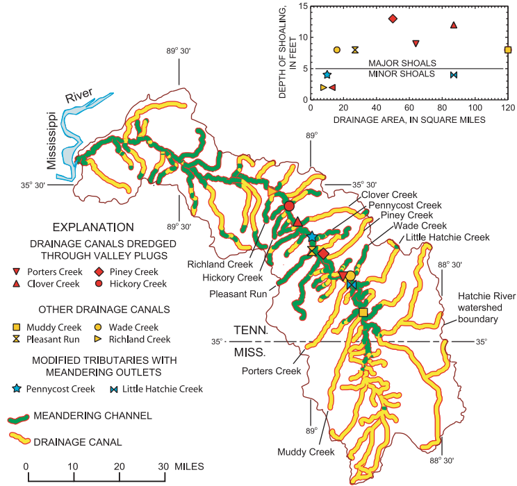
Figure 3. Shoals of the Hatchie River and drainage area of shoal-producing tributaries.
